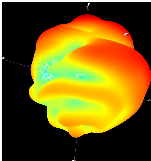
B1.2 3D Pattern for 2440MHz
