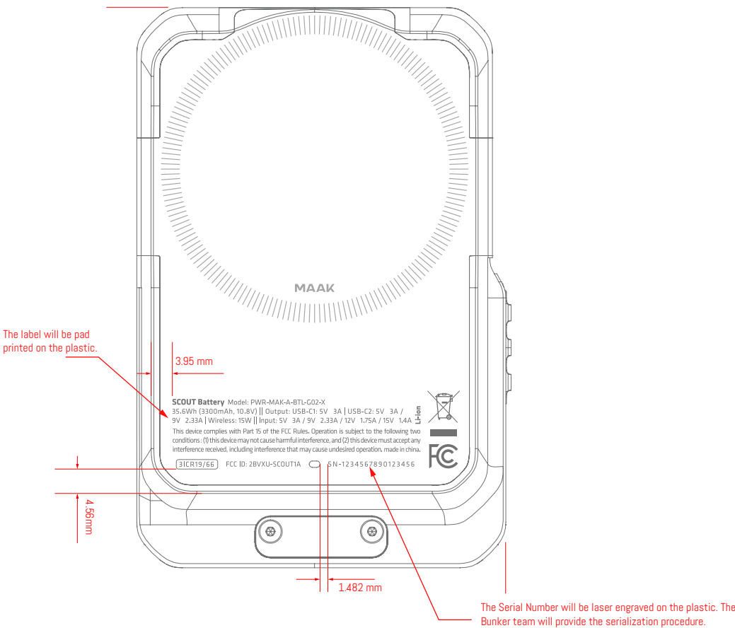
Scout Power Pack - Rear View Position of the Label SCALE 1:1
