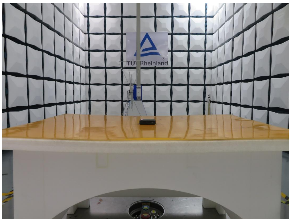
Photograph 2: Set-up photo for Radiated Spurious Emission, Below 1GHz
