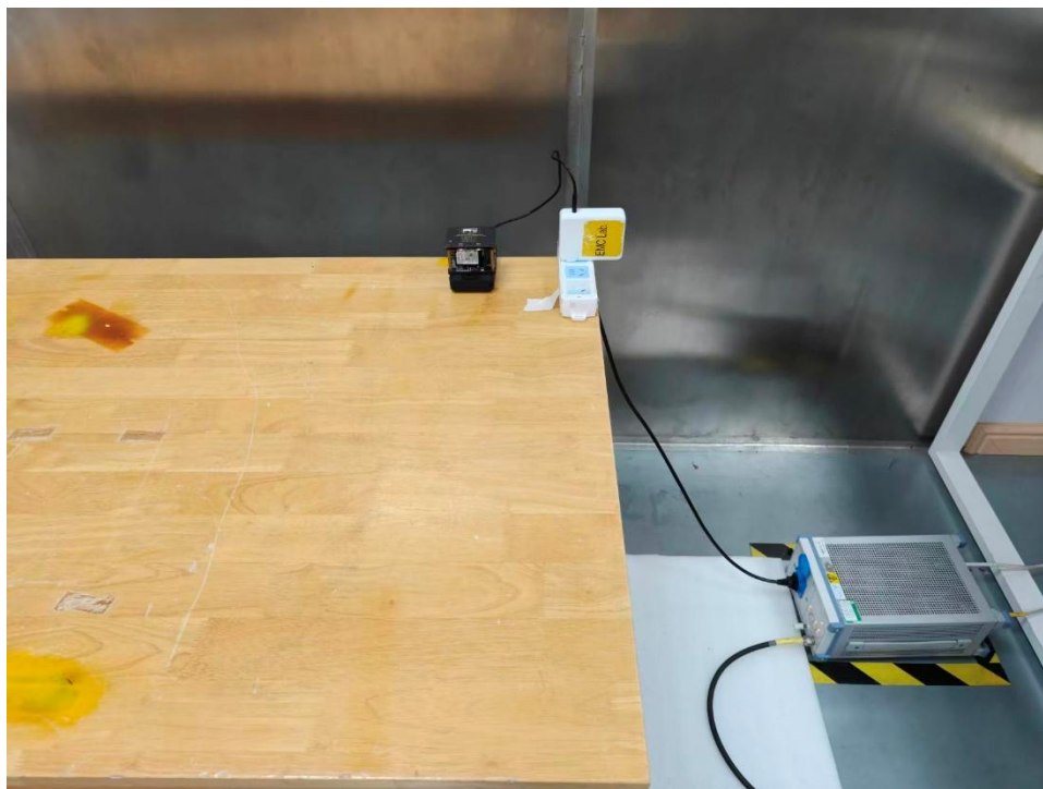
Photograph 1: Set-up photo for Conducted Emission on AC Mains
