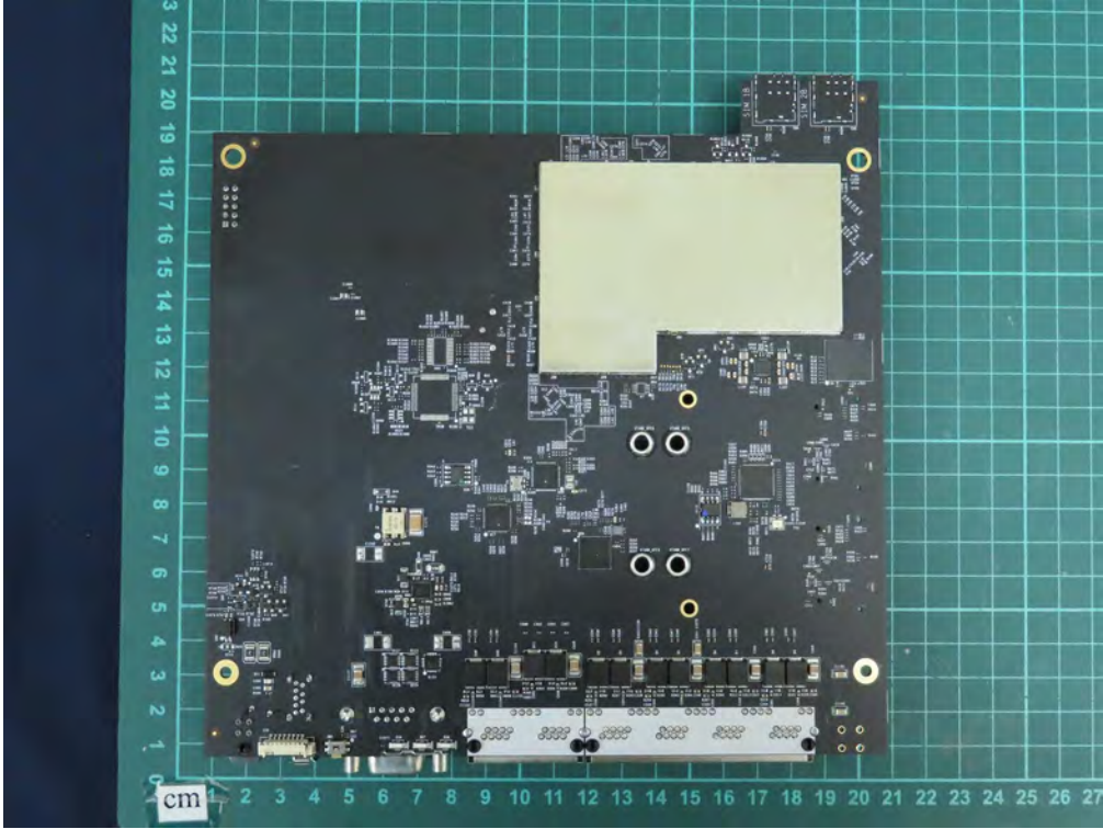
(79) EUT Photo
