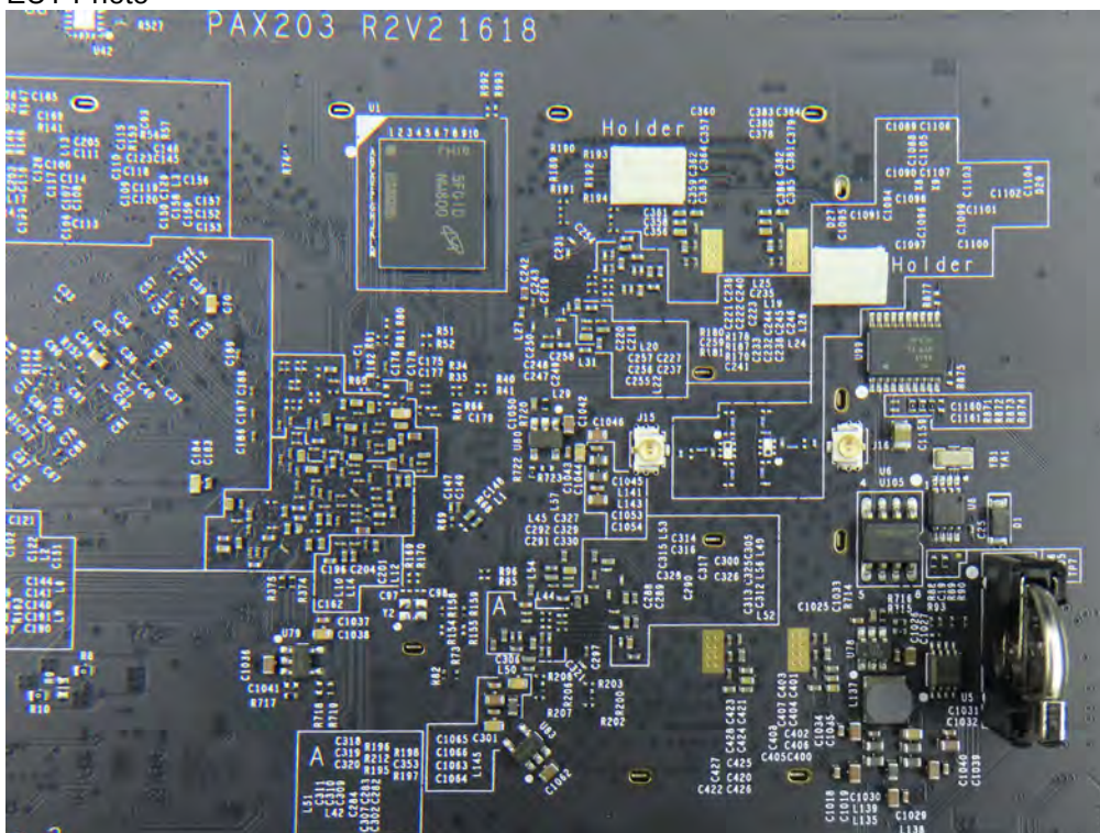
(73) EUT Photo
