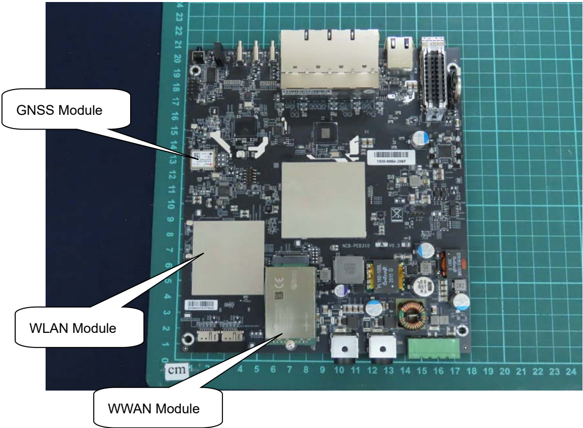
(34) EUT Photo
