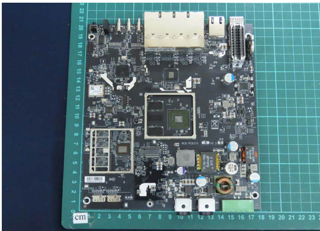
(38) EUT Photo
