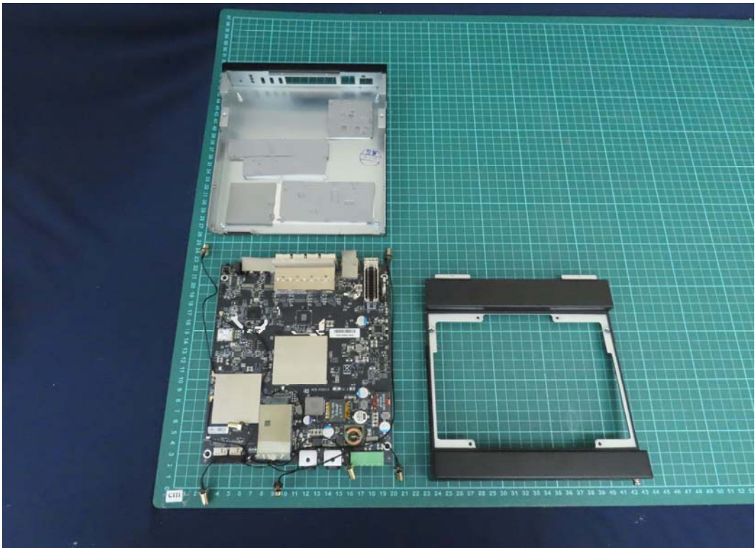
(34) EUT Photo
