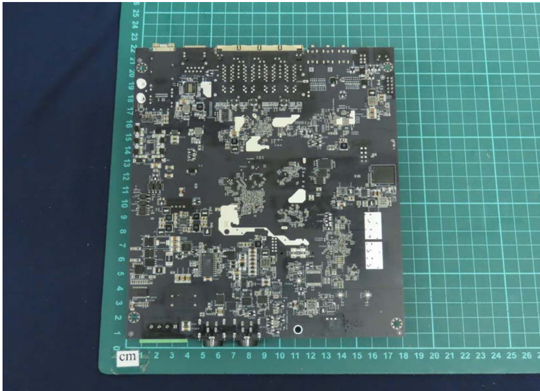
(51) EUT Photo
