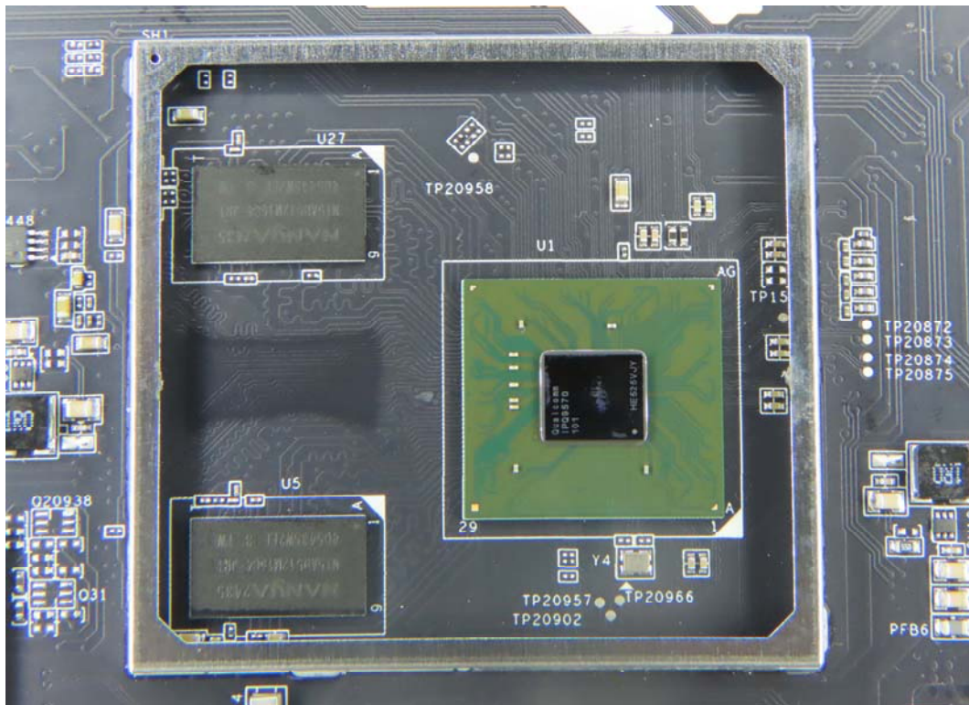
(42) EUT Photo
