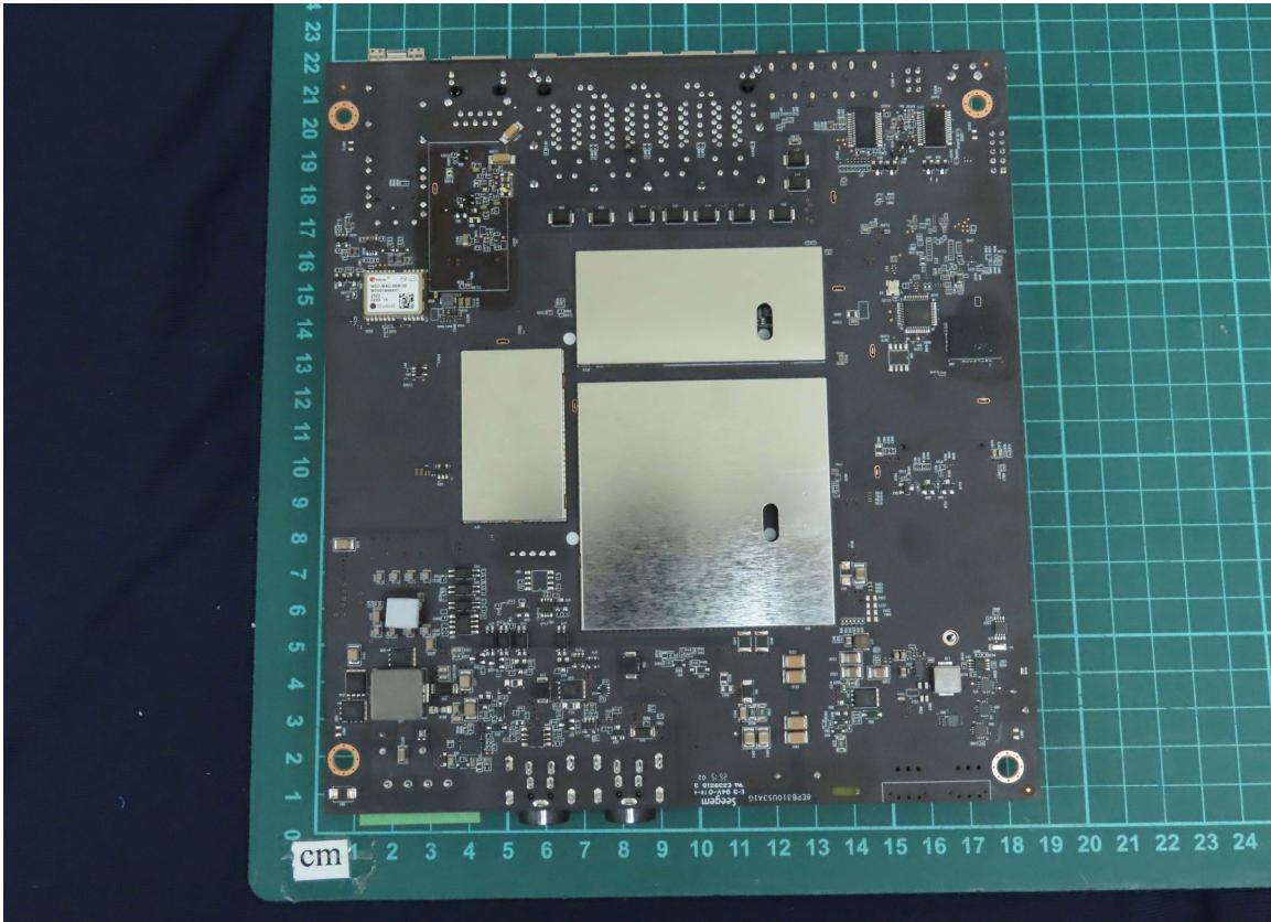
(25) EUT Photo
