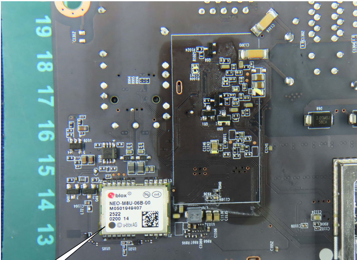
(28) EUT Photo
