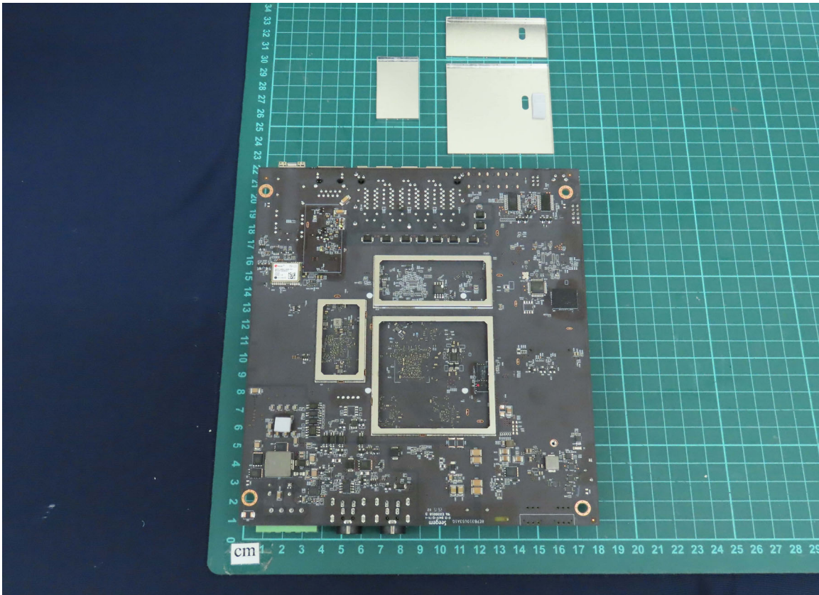
(26) EUT Photo
