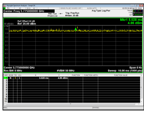
(802.11ac80) plot
