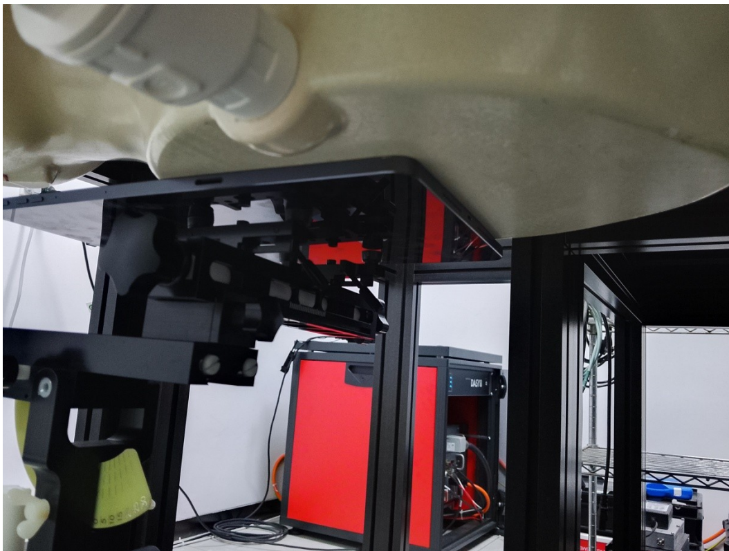
ANT1 Body Back Setup Photo (0 mm)
