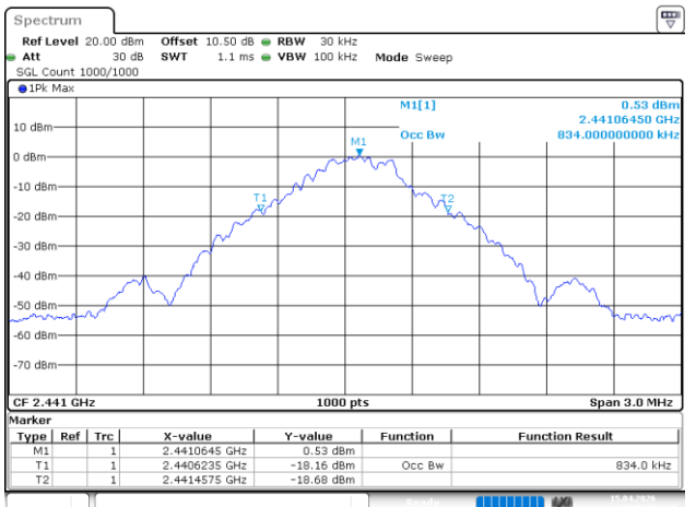
DH5_Middle
