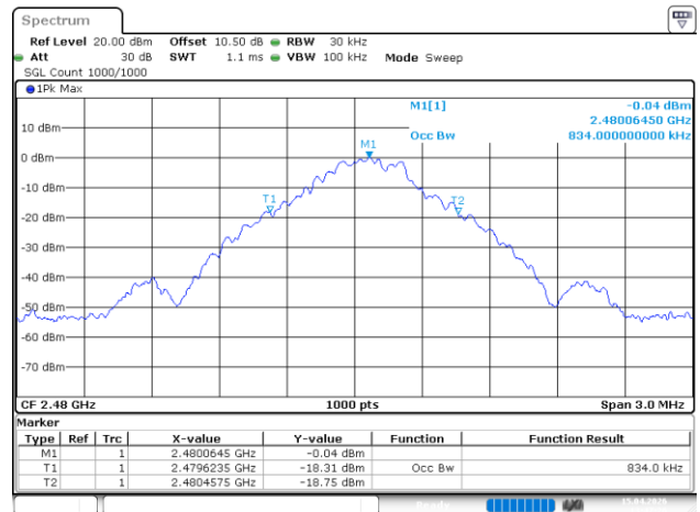
DH5_High
