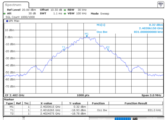
DH5_Low
