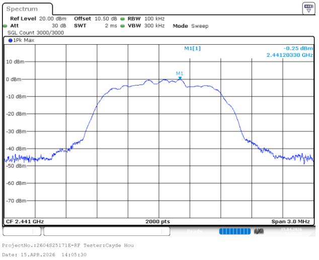
3DH5_Middle
