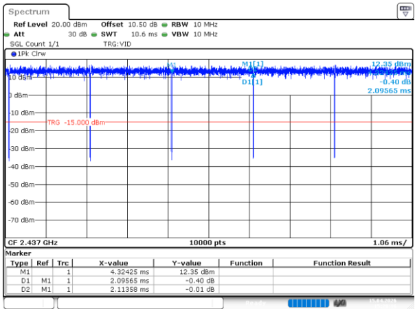
802.11g_2437MHz_Chain 0
