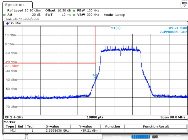
802.11ax20_2412MHz_RU_Full_Chain 0
