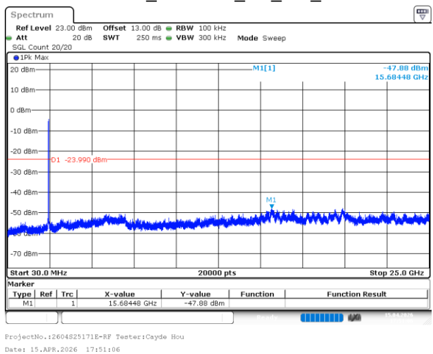
802.11ax40_2452MHz_RU_Full_Chain 1
