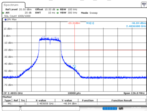
802.11ax20_2462MHz_RU_Full_Chain 1
