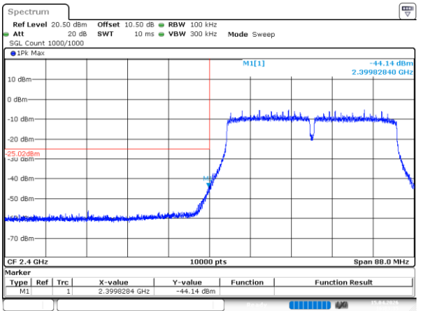
802.11n40_2422MHz_Chain 0
