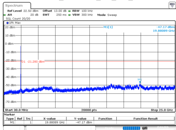
802.11ax20_2437MHz_RU_Full_Chain 1
