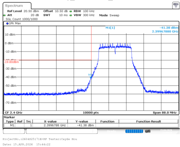
802.11g_2412MHz_Chain 0
