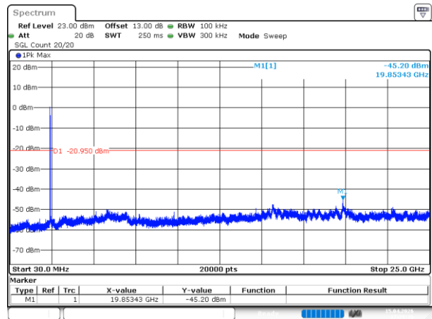
802.11ax20_2412MHz_RU_Full_Chain 1
