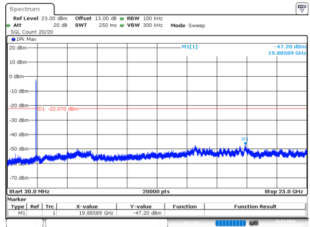
802.11ax20_2412MHz_RU_Full_Chain 0
