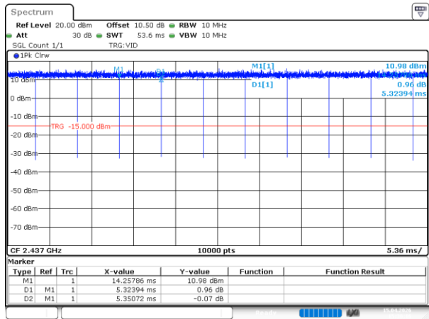
802.11ax20_2437MHz_RU_FULL_Chain 0
