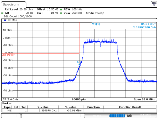
802.11ax20_2412MHz_RU_Full_Chain 1
