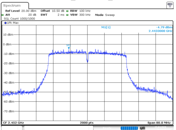
802.11n40_2452MHz_Chain 0
