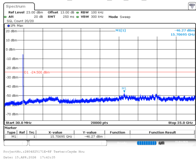
802.11ax40_2437MHz_RU_Full_Chain 1
