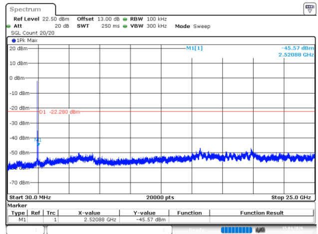
802.11ax20_2437MHz_RU_Full_Chain 0
