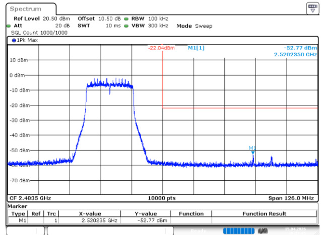
802.11ax20_2462MHz_RU_Full_Chain 0
