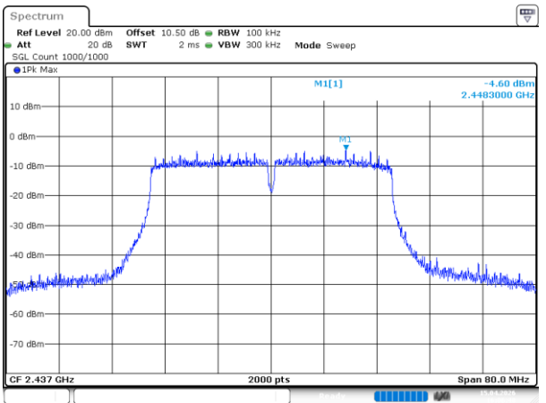
802.11n40_2437MHz_Chain 0
