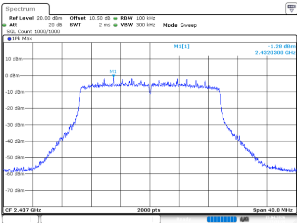
802.11ax20_2437MHz_RU_Full_Chain 1
