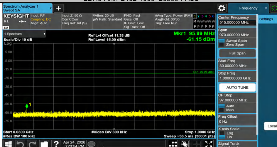
2DH5-Ant1-2441-30~1000-PASS
