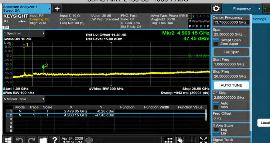
3DH5-Ant1-2480-1000~26500-PASS
