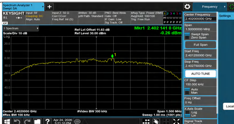
2DH5-Ant1-2402-PASS
