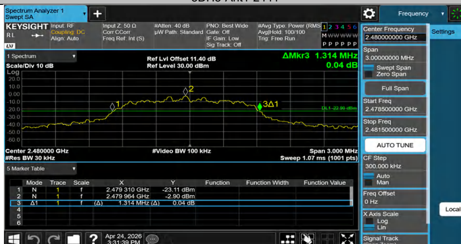
3DH5-Ant1-2480
