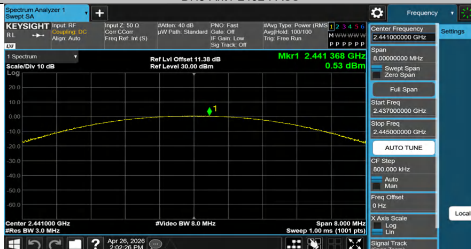
DH5-Ant1-2441-PASS
