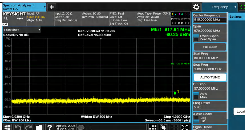
2DH5-Ant1-2402-30~1000-PASS
