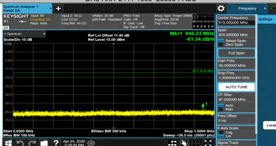
DH5-Ant1-2480-30~1000-PASS
