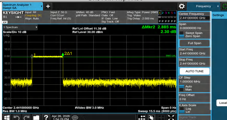
2DH5-Ant1-Hop-PASS
