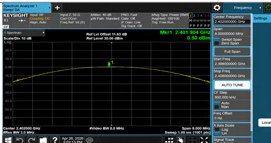
DH5-Ant1-2402-PASS
