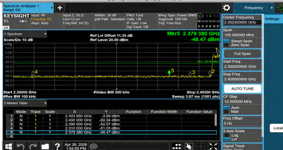
3DH5-Ant1-Hop_2402-PASS
