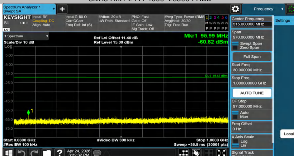
3DH5-Ant1-2480-30~1000-PASS
