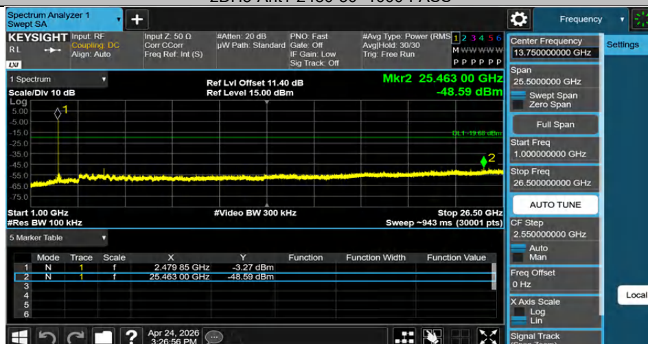
2DH5-Ant1-2480-1000~26500-PASS
