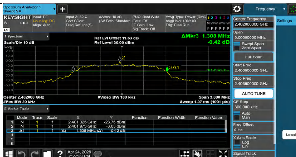
3DH5-Ant1-2402
