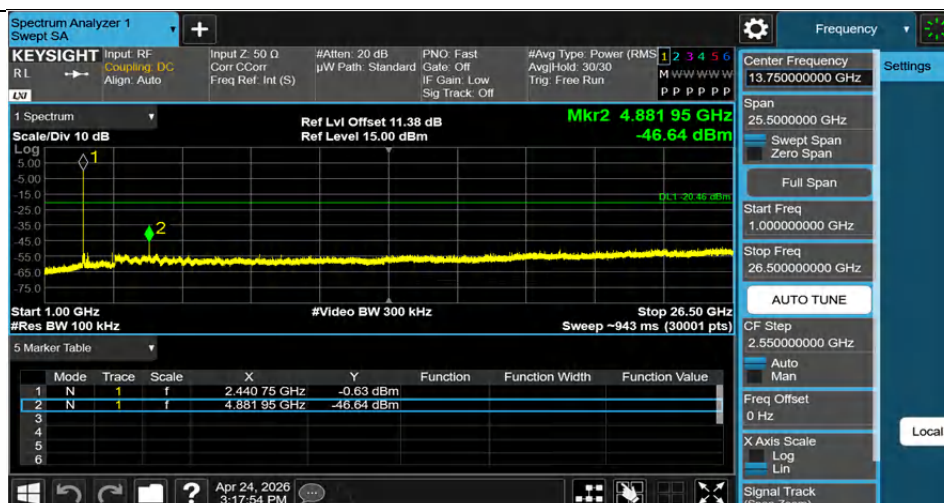
DH5-Ant1-2441-1000~26500-PASS
