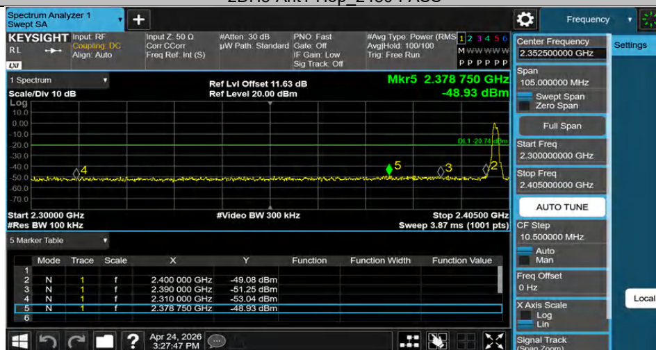
3DH5-Ant1-2402-PASS
