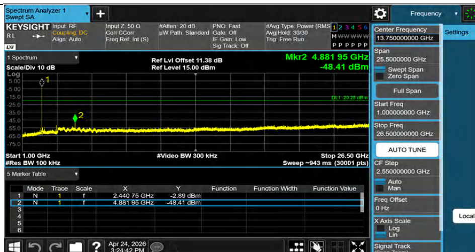
2DH5-Ant1-2441-1000~26500-PASS
