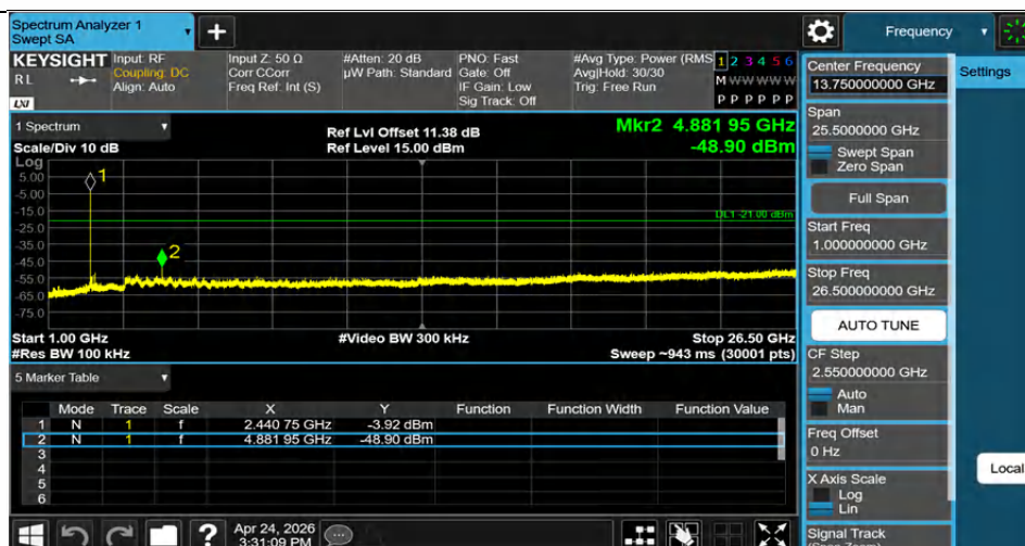
3DH5-Ant1-2441-1000~26500-PASS
