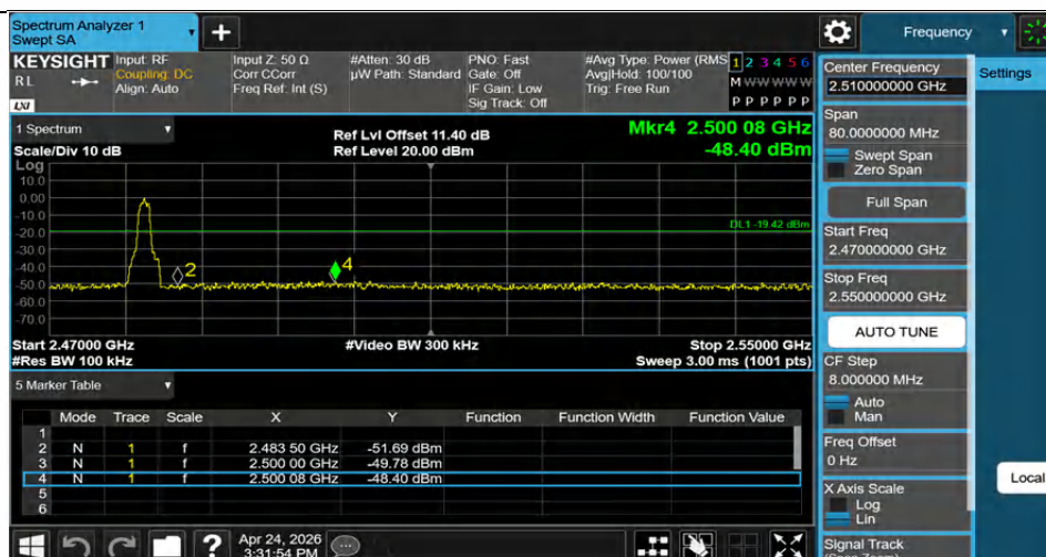
3DH5-Ant1-2480-PASS
