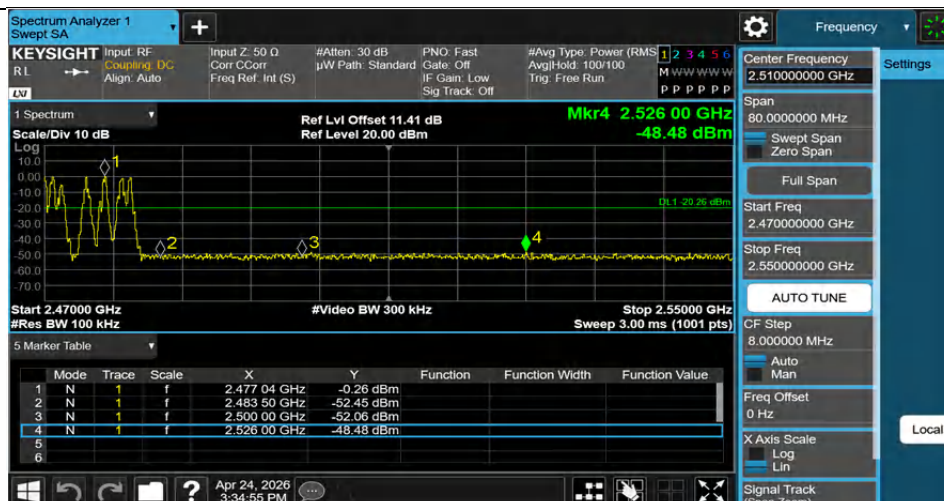
DH5-Ant1-Hop_2480-PASS
