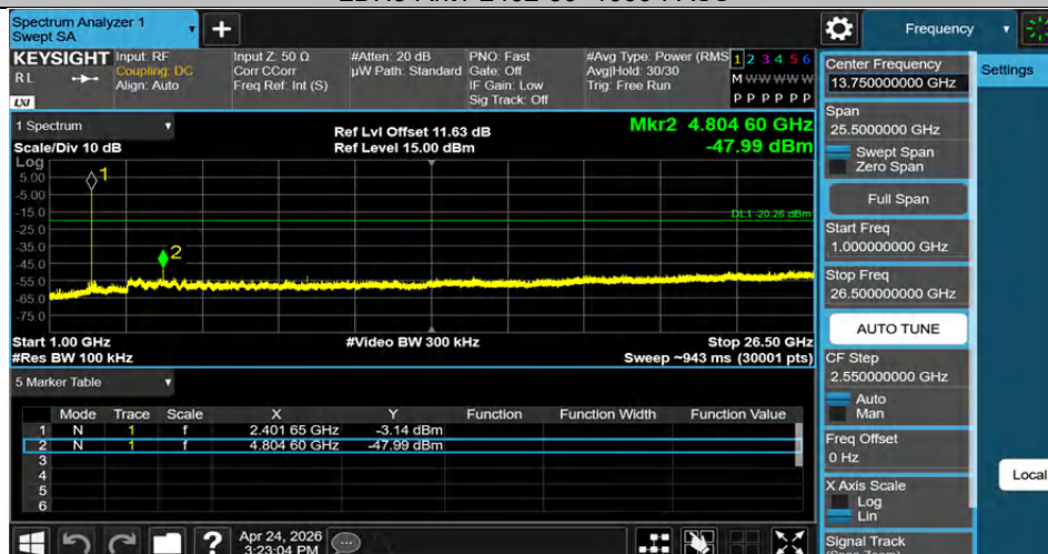
2DH5-Ant1-2402-1000~26500-PASS
