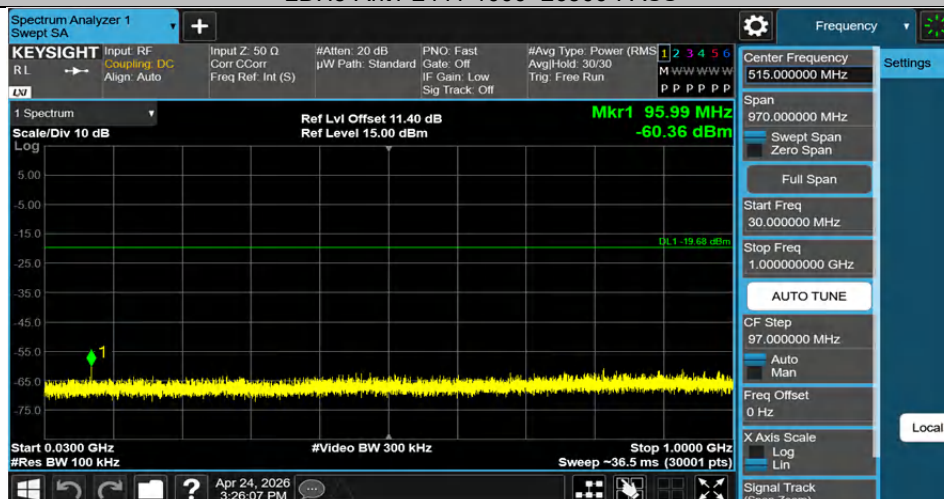
2DH5-Ant1-2480-30~1000-PASS
