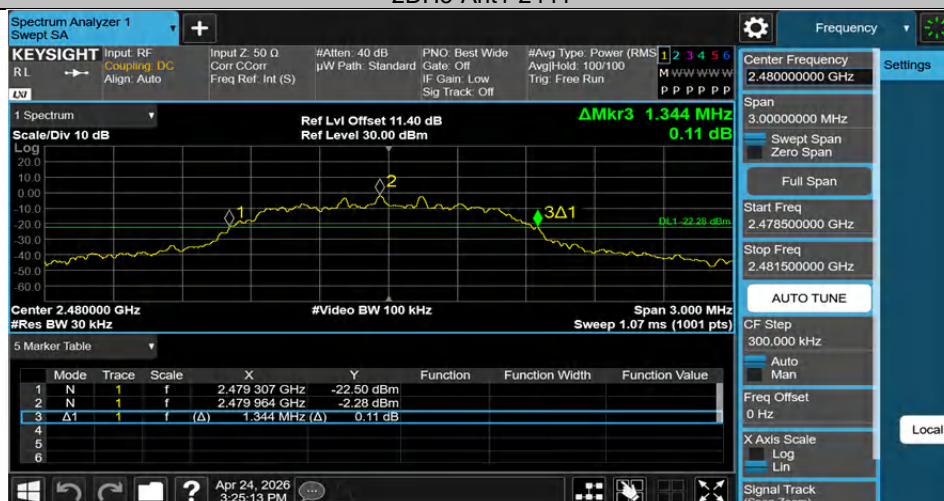
2DH5-Ant1-2480
