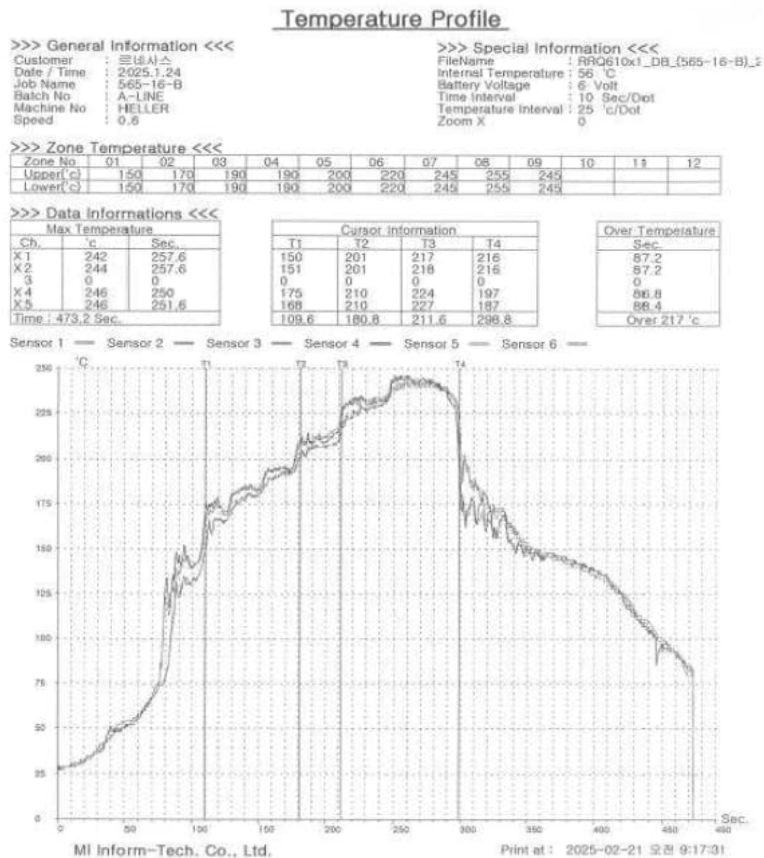
Figure 29. Reflow profile for lead free solder, applied on RRQ61001 daughterboard
