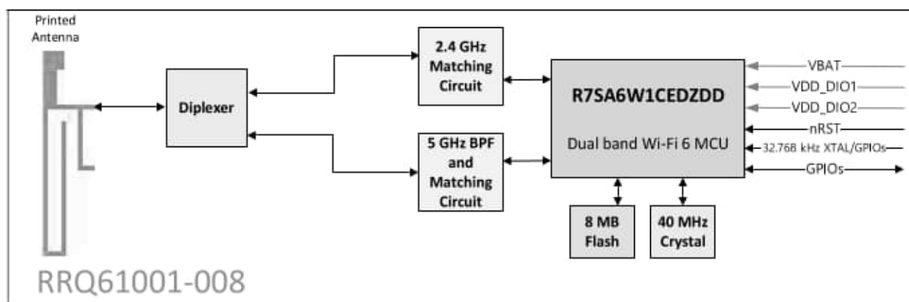
Figure 1. Interconnection of all the physical blocks in RRQ61001-008 module
