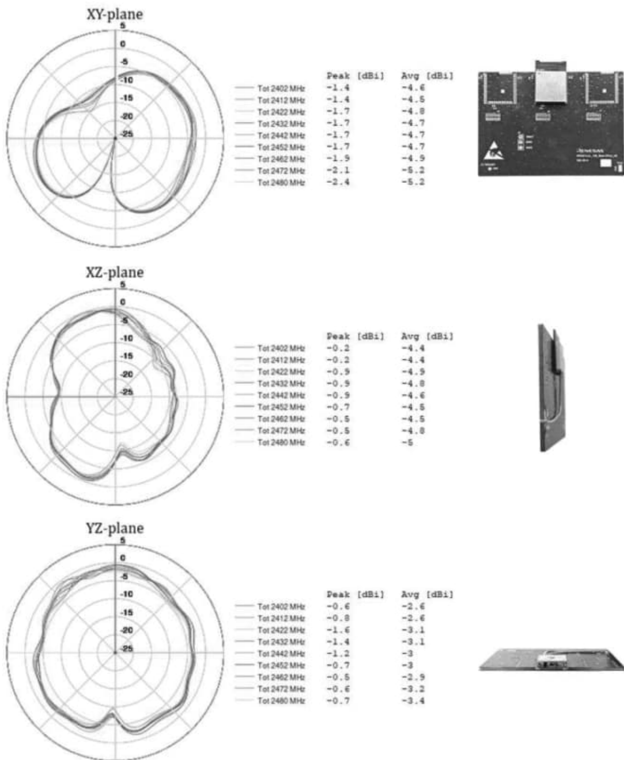
Figure 21. 2D radiation patterns for 2.4 GHz band for RRQ61001-008 module
