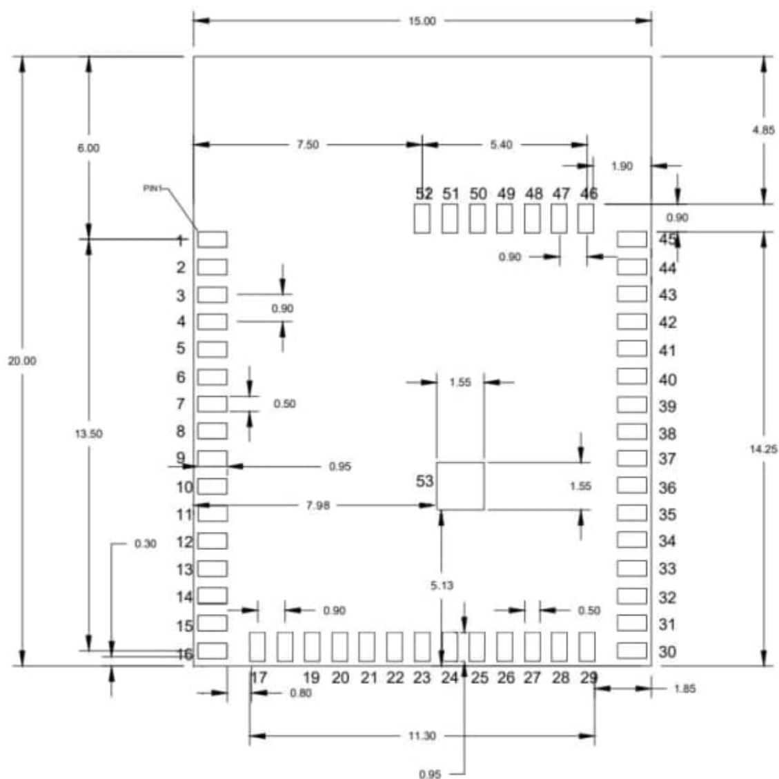
Figure 25. Recommended land pattern (PCB top view, NSMD design)
