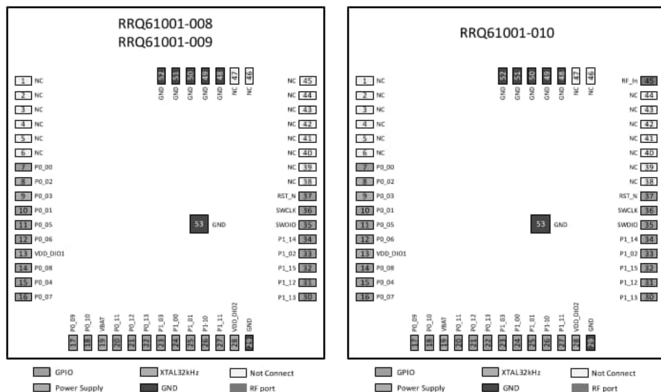
Figure 5. RRQ61001 pinout
