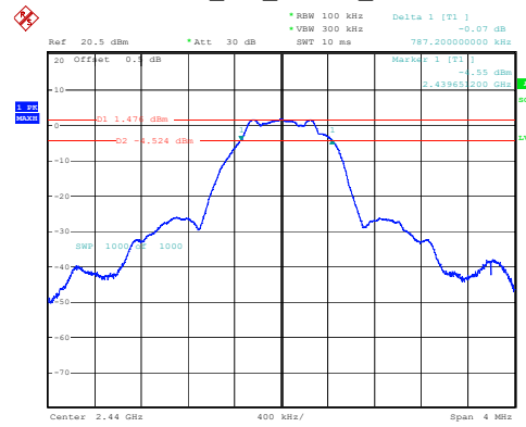
BLE_1M_Middle_Channel
