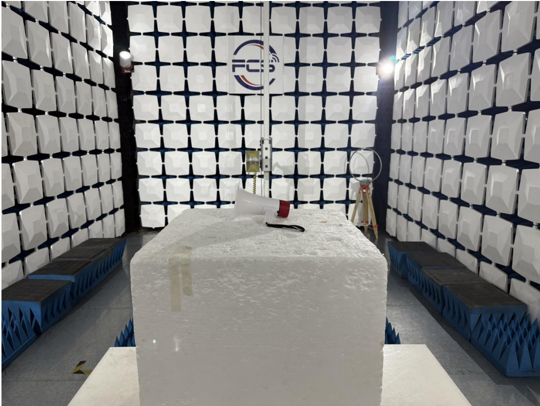
RE (Above1GHz)
