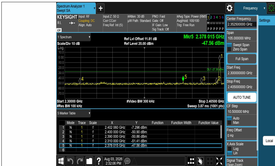
DH5-Ant1-2402-PASS
