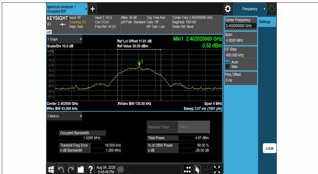
BLE_1M-Ant1-2402
