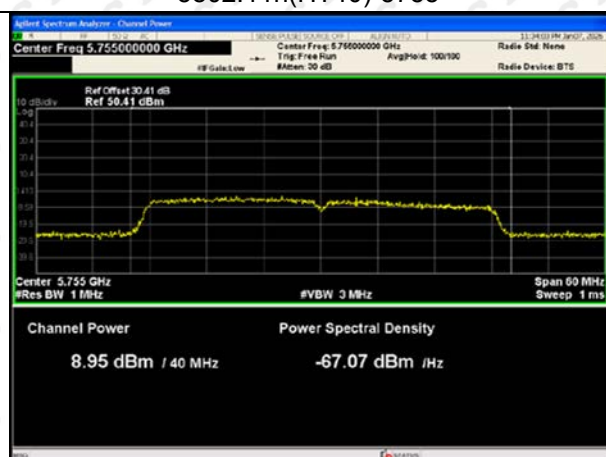
5802.11n(HT40)-5755
