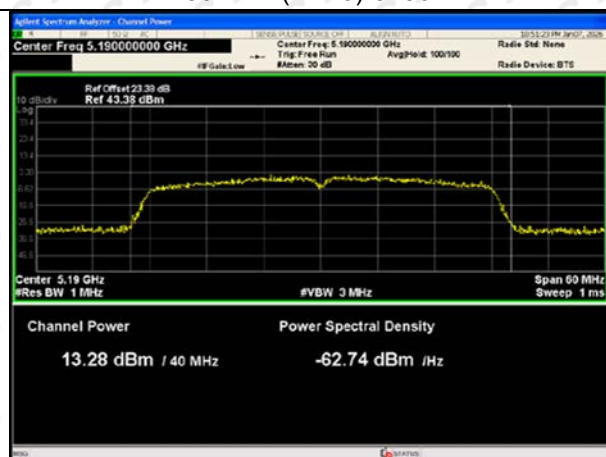
802.11n(HT40)-5190
