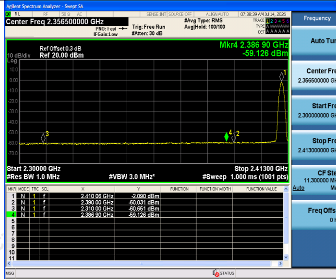
2.4G Ant1 Low 2410 Peak
