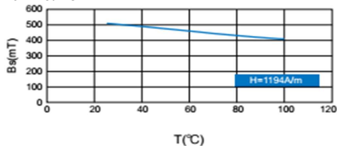
Bs—T Curve
