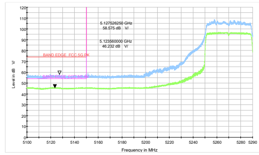
802.11ax HE40-484-Tone-Channel 54: Peak + Average
