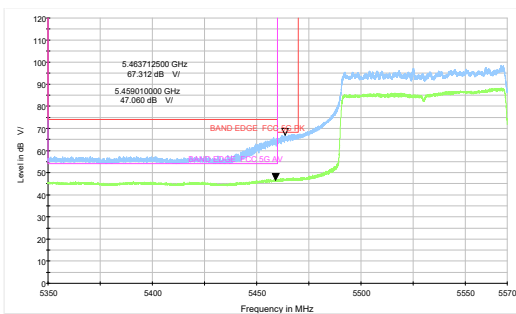
802.11ax HE80-996-Tone-Channel 106: Peak + Average
