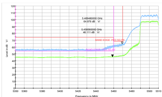
802.11ax HE20-242-Tone-Channel 100: Peak + Average
