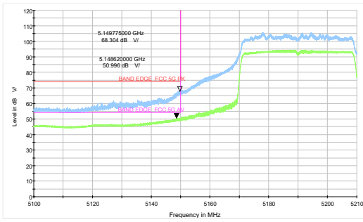
802.11ax HE40-484-Tone-Channel 38: Peak + Average
