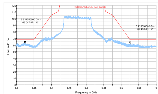
802.11ax HE80-996-Tone-Channel 155: Peak
