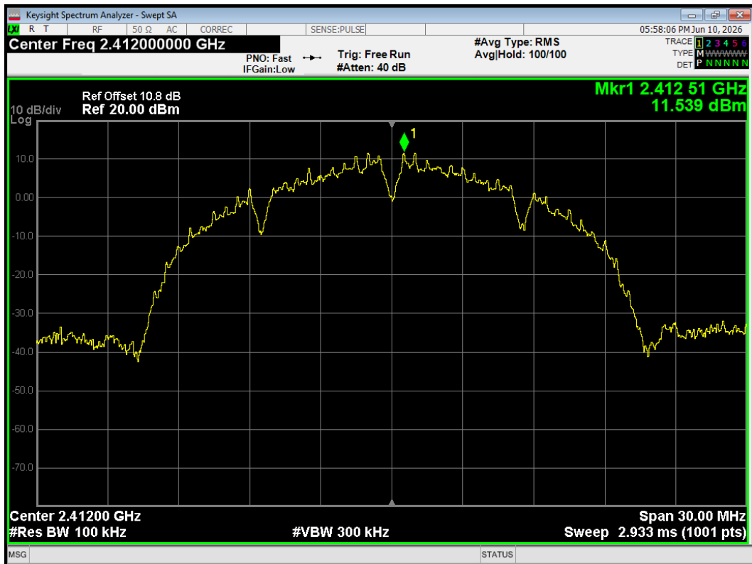
Tx. Spurious 802.11b 2412MHz Emission
