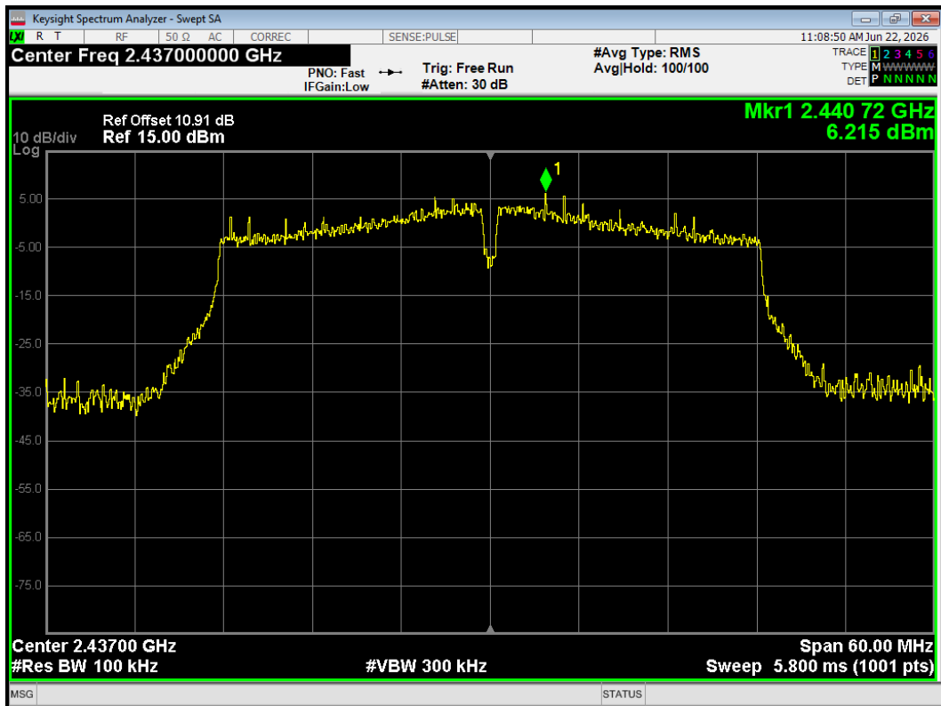
Tx. Spurious 802.11n(HT40) 2437MHz Emission
