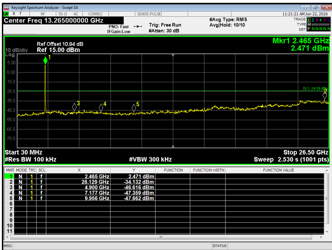
Tx. Spurious 802.11n(HT40) 2452MHz Emission
