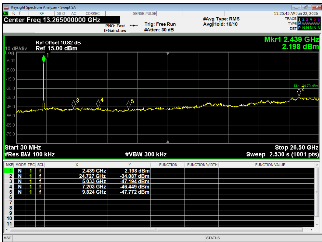
Tx. Spurious 802.11ax(HE40) 2437MHz Ref
