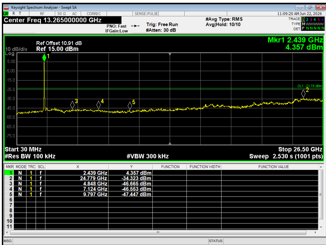
Tx. Spurious 802.11n(HT40) 2452MHz Ref
