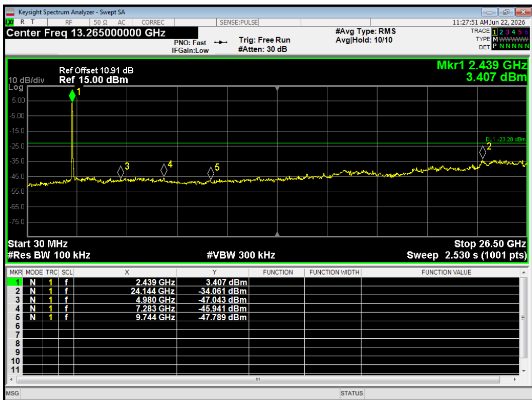
Tx. Spurious 802.11ax(HE40) 2452MHz Ref
