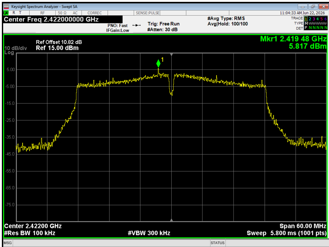
Tx. Spurious 802.11n(HT40) 2422MHz Emission
