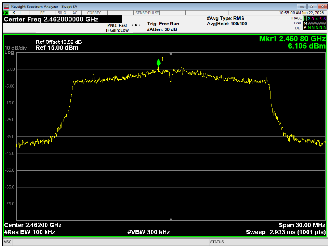
Tx. Spurious 802.11ax(HE20) 2462MHz Emission
