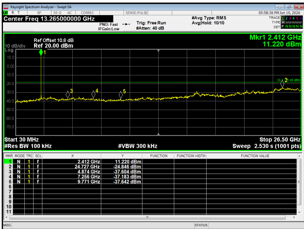
Tx. Spurious 802.11b 2437MHz Ref
