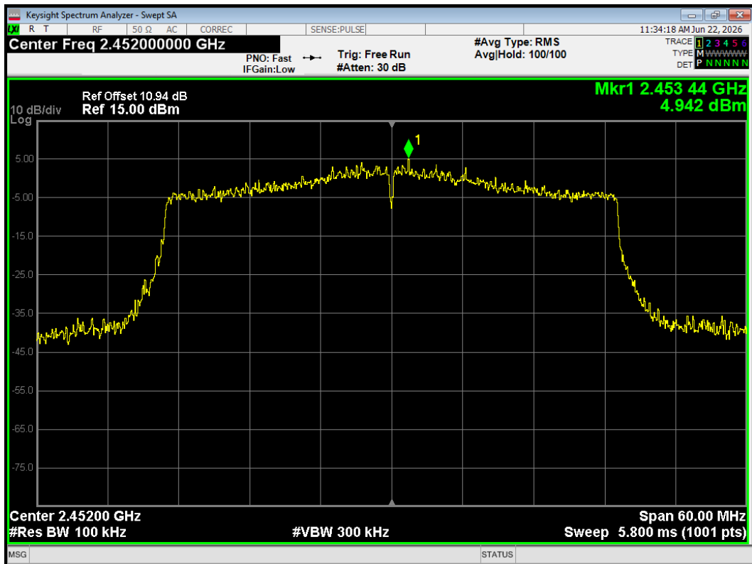
Tx. Spurious 802.11ax(HE40) 2452MHz Emission
