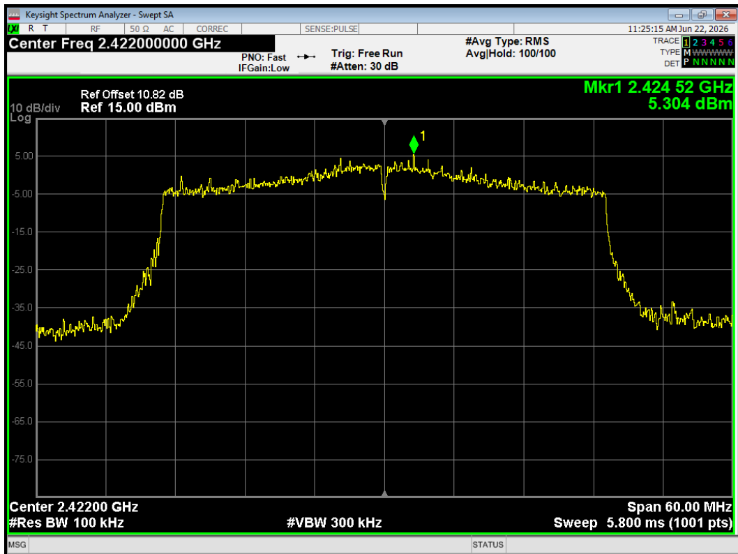
Tx. Spurious 802.11ax(HE40) 2422MHz Emission
