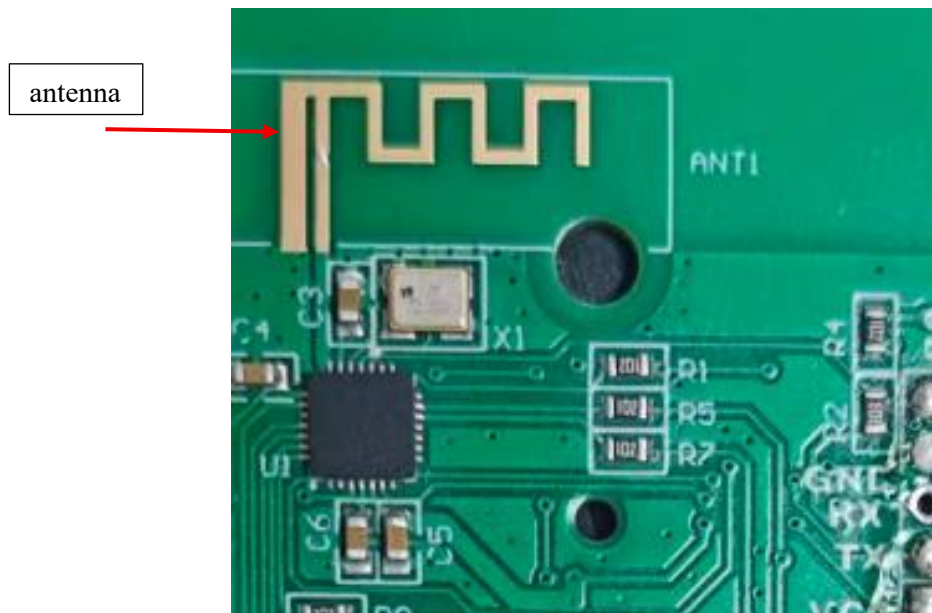
Antenna design
