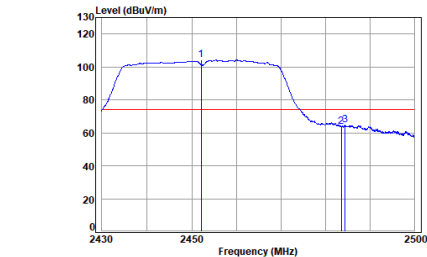
11n_HT(40M)_TX_CH_09_Horizontal-Peak
