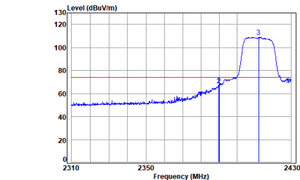
11g_TX_CH_01_Vertical-Peak
