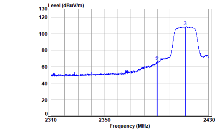
11g_TX_CH_01_Horizontal-Peak
