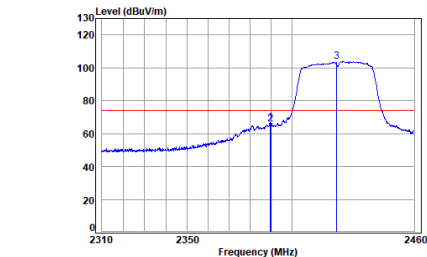
11n_HT(40M)_TX_CH_03_Vertical-Peak
