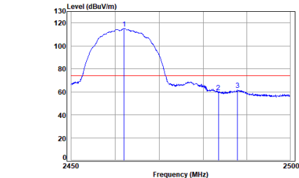
11b_TX_CH_11_Vertical-Peak
