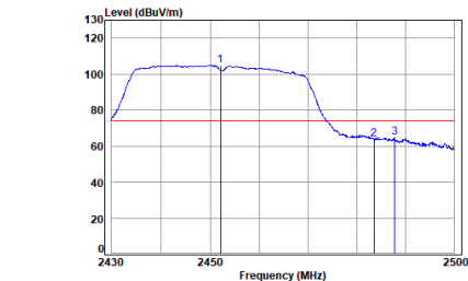
11n_HT(40M)_TX_CH_09_Vertical-Peak
