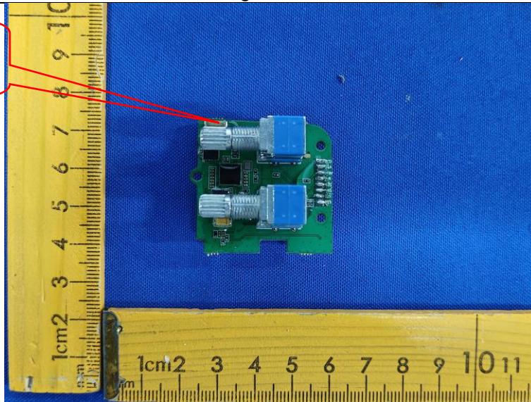
Chip Antenna
