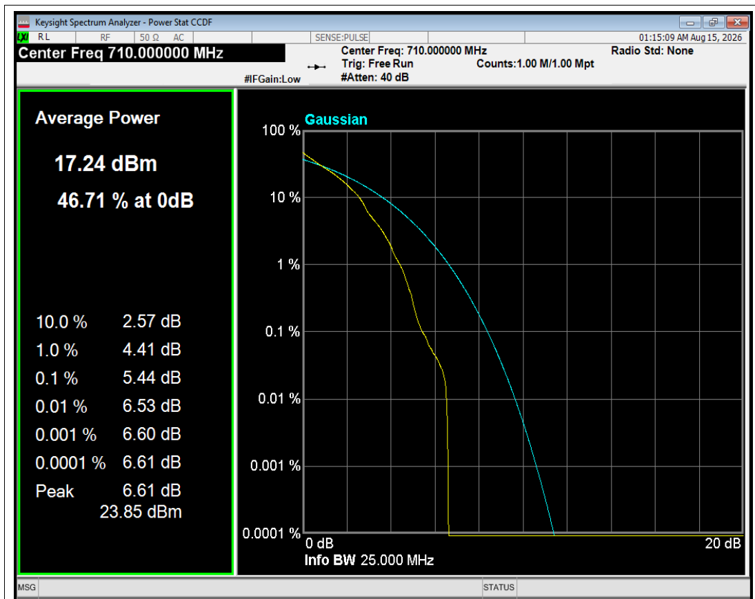
Band17 64QAM BW=10MHz Channel=23790 RB Size=1 Position=#0 NVNT
