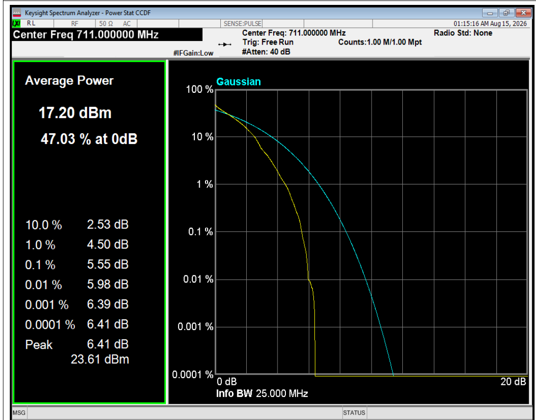
Band17 QPSK BW=10MHz Channel=23800 RB Size=1 Position=#0 NVNT
