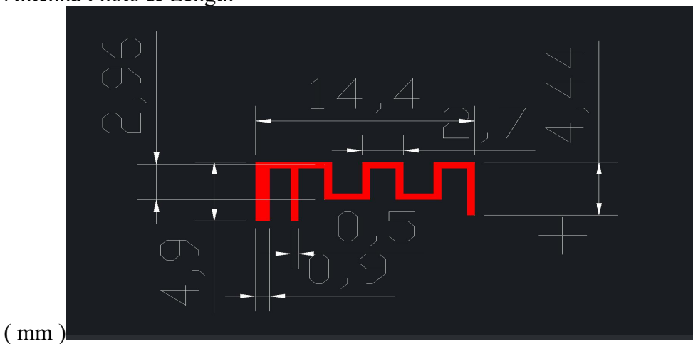
Antenna Photo & Length
