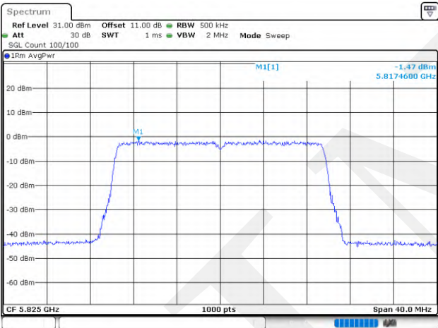
802.11ax20_5825MHz_RU_Full_Chain 0
