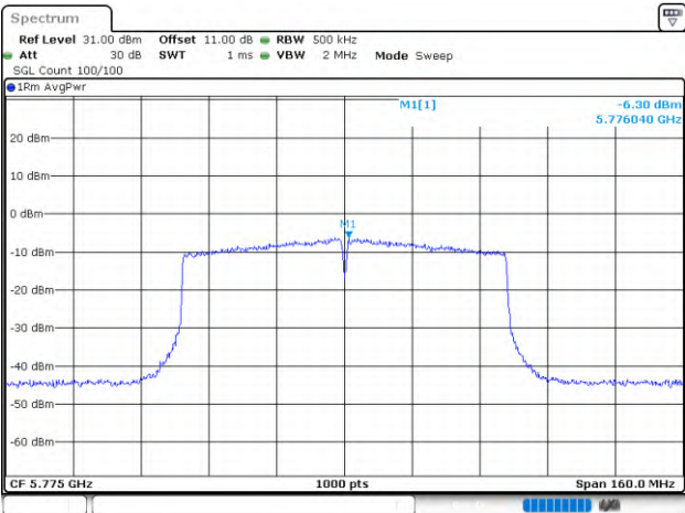
802.11ac80_5775MHz_Chain 1
