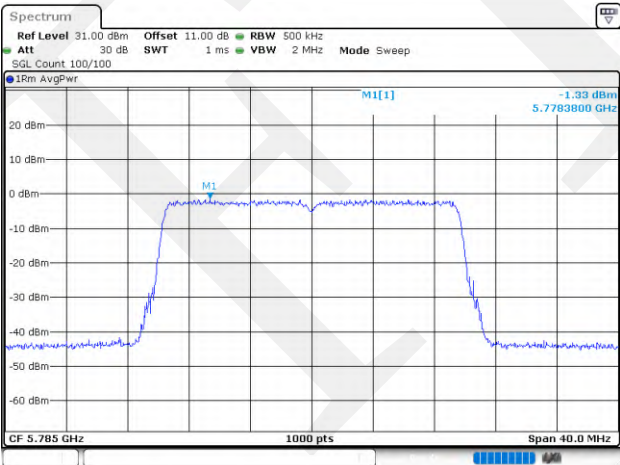
802.11ax20_5785MHz_RU_Full_Chain 1
