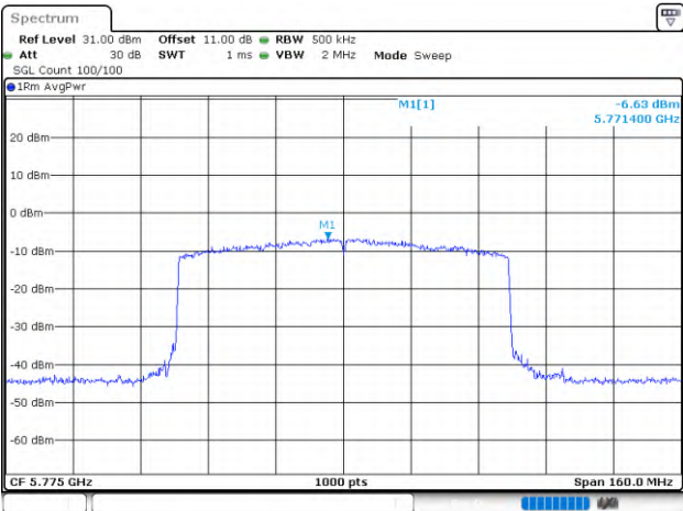
802.11ax80_5775MHz_RU_Full_Chain 1
