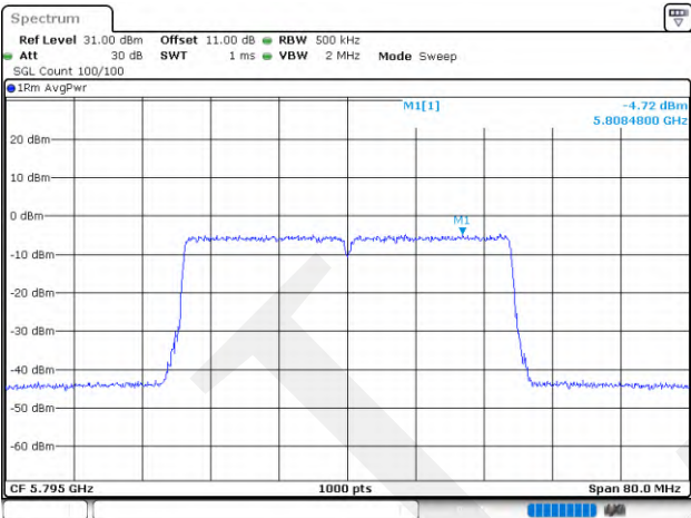
802.11ax40_5795MHz_RU_FULL_Chain 0
