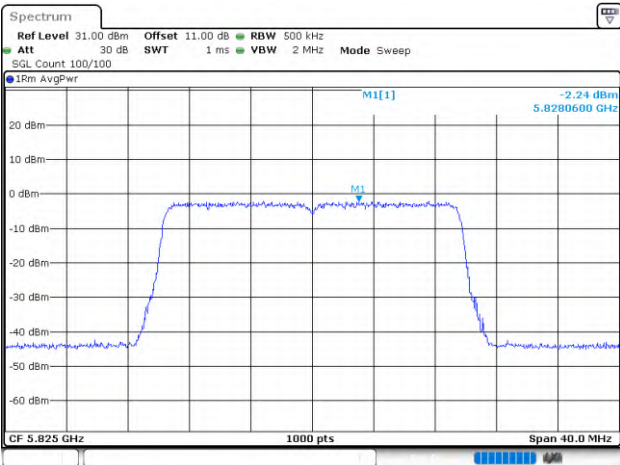
802.11ax20_5825MHz_RU_Full_Chain 1
