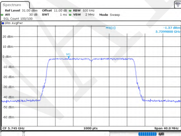
802.11ax20_5745MHz_RU_Full_Chain 1
