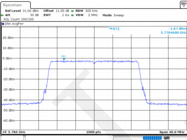
802.11ax20_5785MHz_RU_Full_Chain 0
