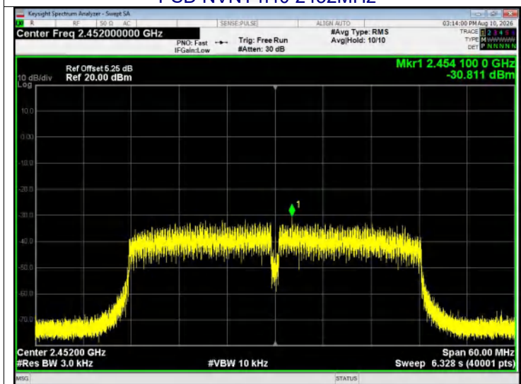
PSD NVNT n40 2452MHz
