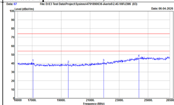
TX, 802.11b - Emission (Ch 6) Radiated Spurious Emission, Vertical
