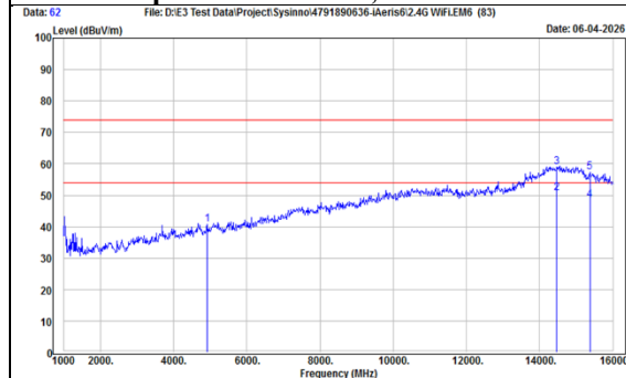
TX, 802.11g - Emission (Ch 11) Radiated Spurious Emission, Horizontal
