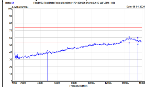
TX, 802.11b - Emission (Ch 6) Radiated Spurious Emission, Horizontal
