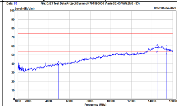
TX, 802.11g - Emission (Ch 11) Radiated Spurious Emission, Vertical
