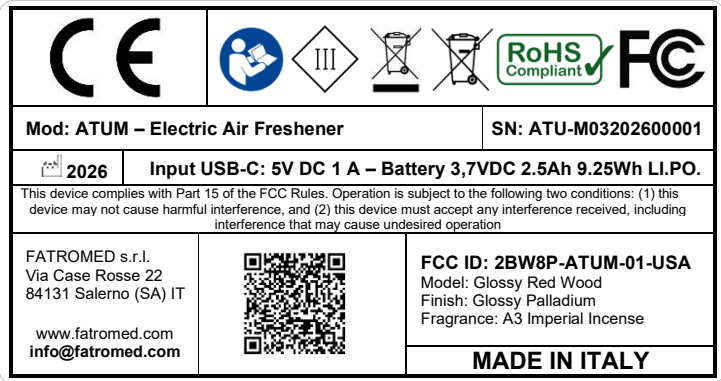
Picture 3: Packaging label drawing (actual size)
