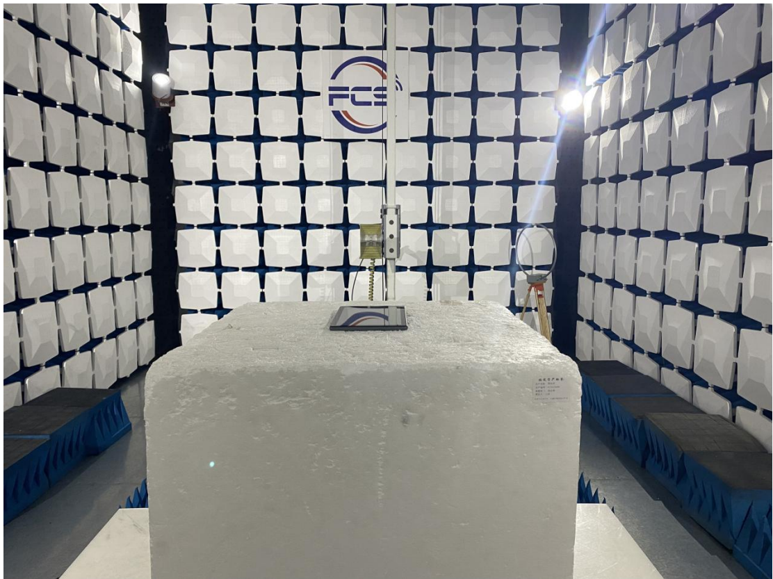
RE (Above1GHz)
