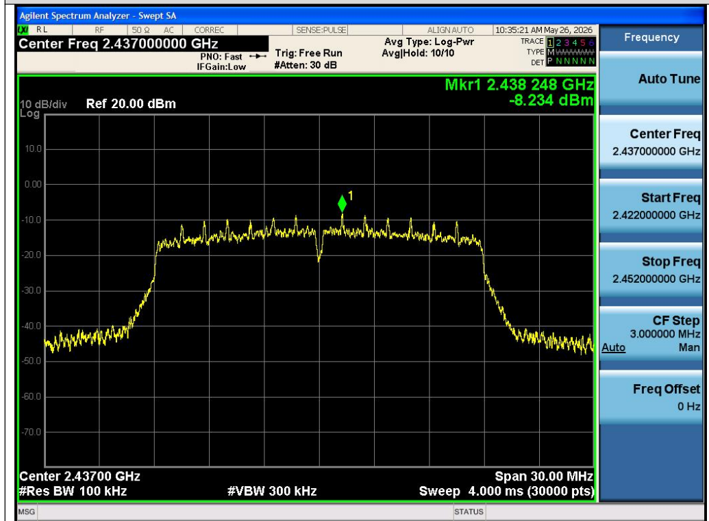
Test_Graph_802.11n20_ANT1_2437_MCS0_Reference Level
