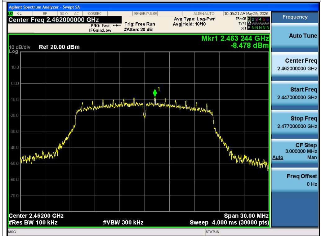
Test_Graph_802.11g_ANT1_2462_6Mbps_Reference Level
