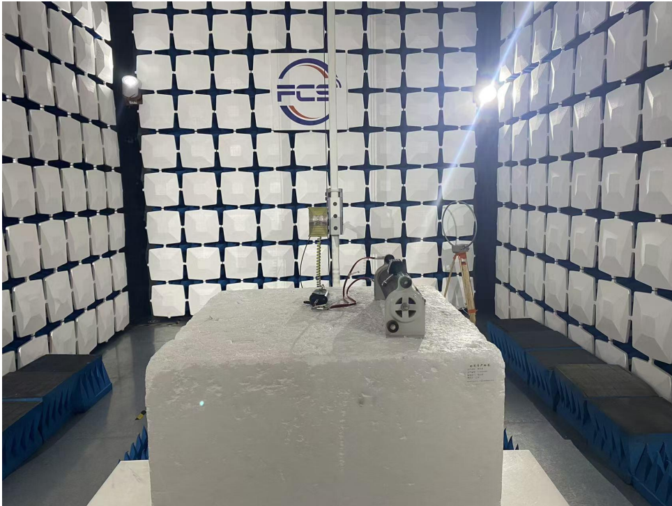
RE (Above1GHz)
