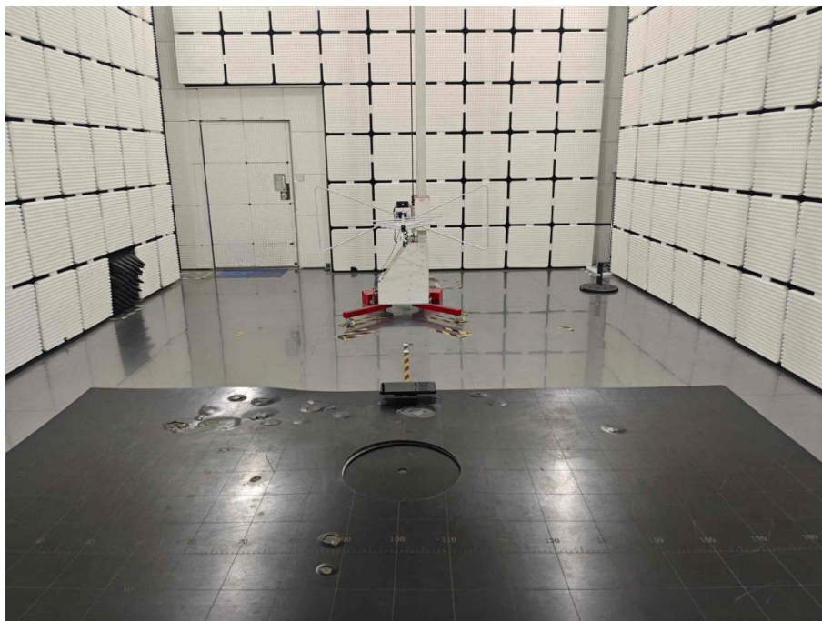
Emissions in Non-restricted Frequency Bands(Blow 30 MHz)
