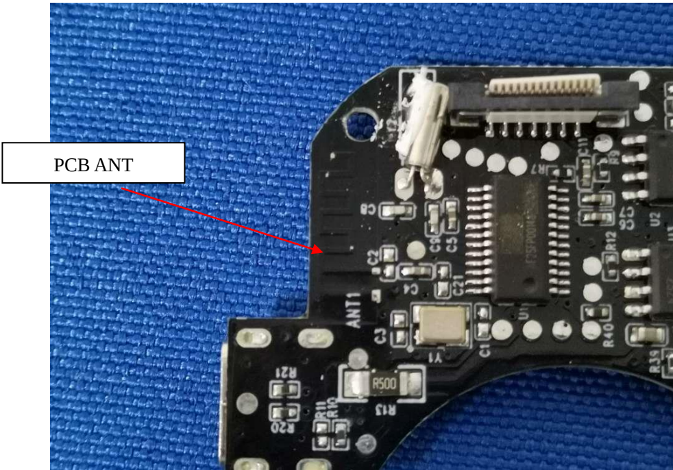
EUT Internal View 6
