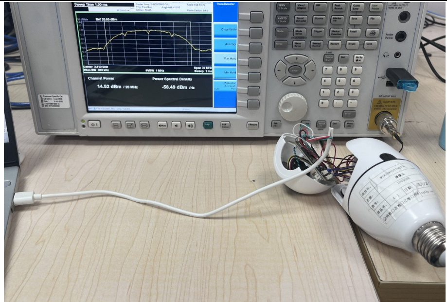
Radio Test Setup View
