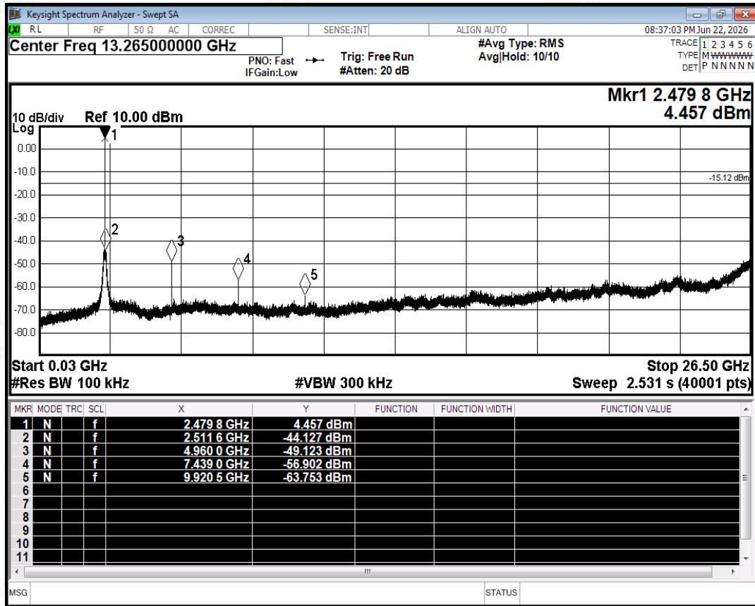
Tx. Spurious NVNT 2.4G 2480MHz Ant1 Emission
