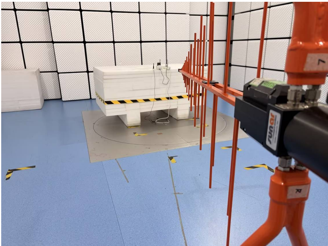
Radiation Emission_ Below 1GHz - Back View
