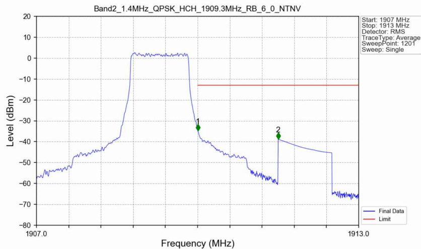
Band2_1.4MHz_QPSK_HCH_1909.3MHz_RB_6_0_NTNV
