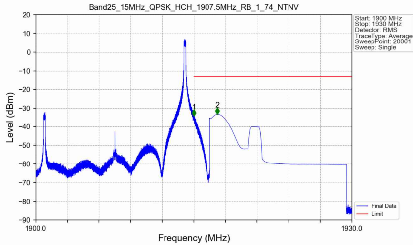
Band25_15MHz_QPSK_HCH_1907.5MHz_RB_1_74_NTNV
