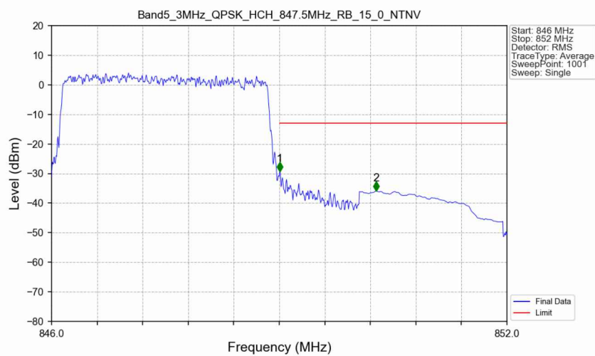
Band5_3MHz_QPSK_HCH_847.5MHz_RB_15_0_NTNV
