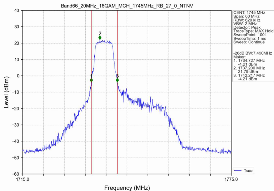
Band66_20MHz_16QAM_MCH_1745MHz_RB_27_0_NTNV
