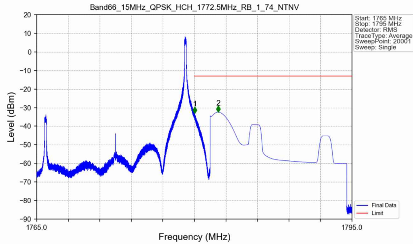
Band66_15MHz_QPSK_HCH_1772.5MHz_RB_1_74_NTNV
