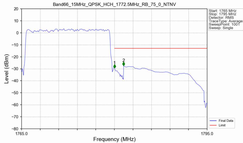
Band66_15MHz_QPSK_HCH_1772.5MHz_RB_75_0_NTNV
