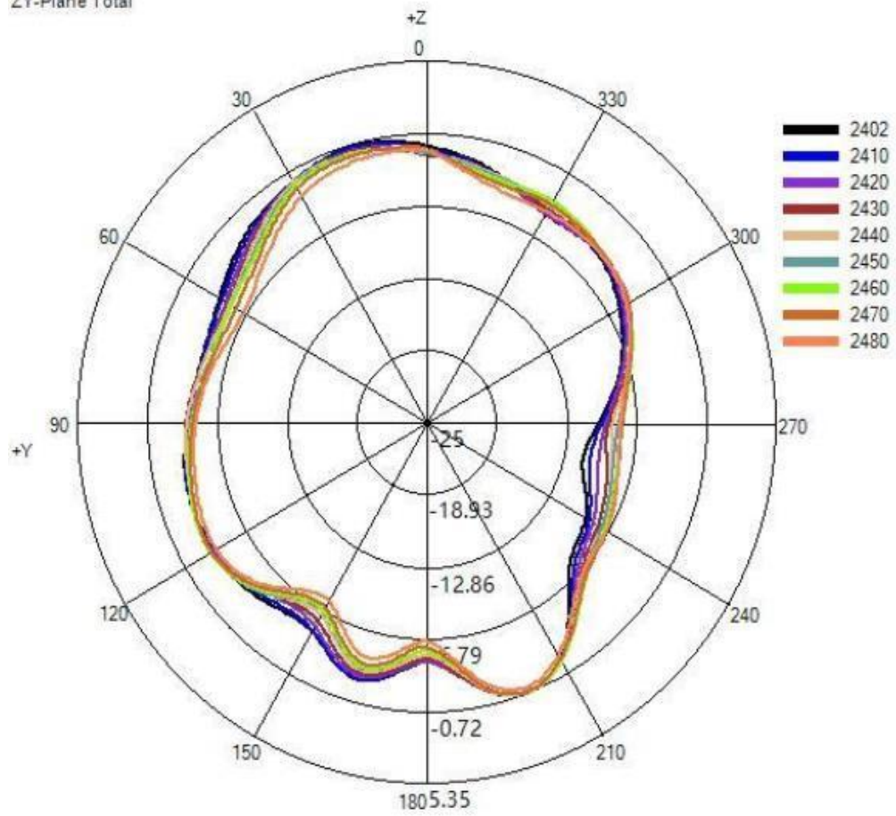
ZY-Plane Total
