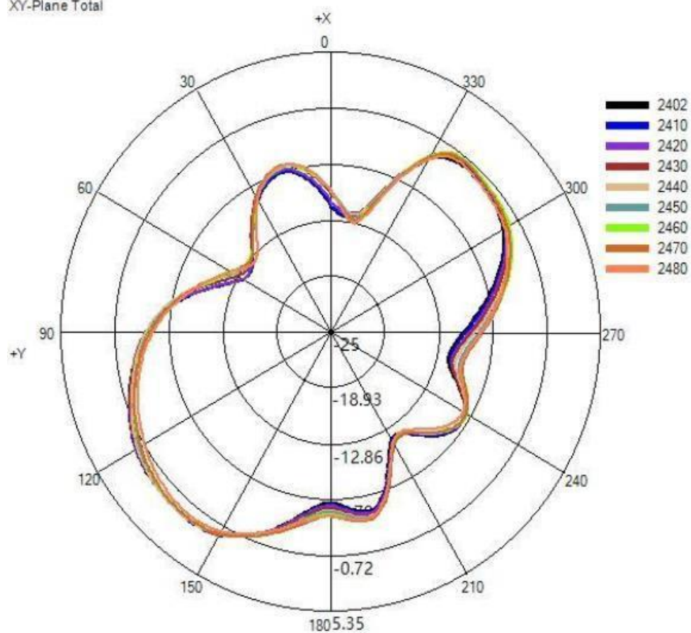
XY-Plane Total
