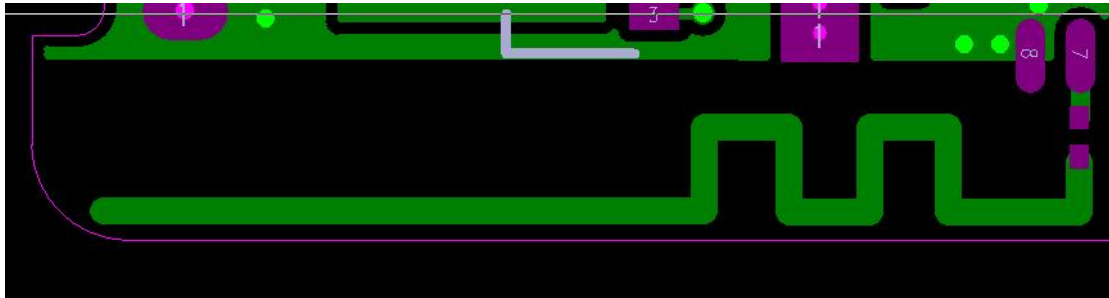
Antenna shape
