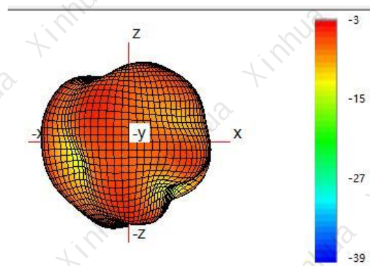
(6) Typical Free Space 3D Radiation Pattern at 2500MHz(unit:dBi)
