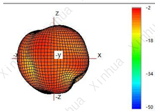
(5) Typical Free Space 3D Radiation Pattern at 2450MHz(unit:dBi)
