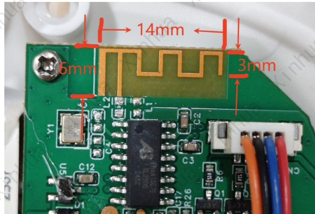
Antenna Dimensions
