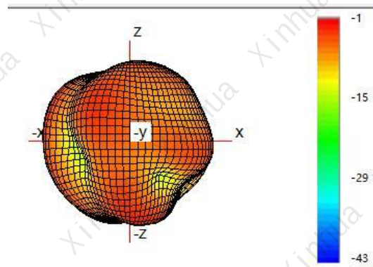
(4) Typical Free Space 3D Radiation Pattern at 2400MHz(unit:dBi)
