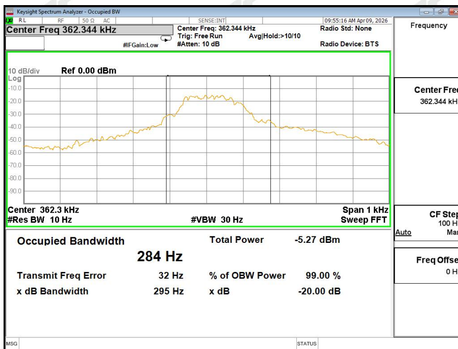
360KHz Coil ANT
