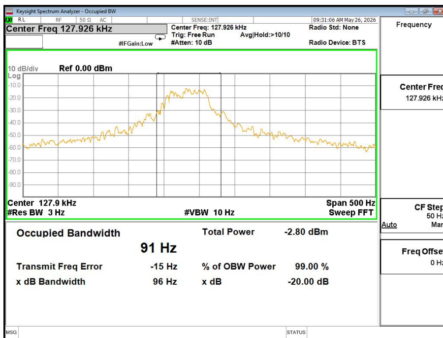
111-205KHz Coil Antenna 1
