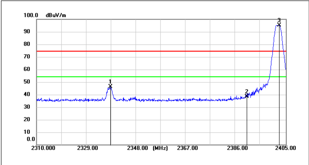
BLE_2M_TX_CH_00_Horizontal_Peak
