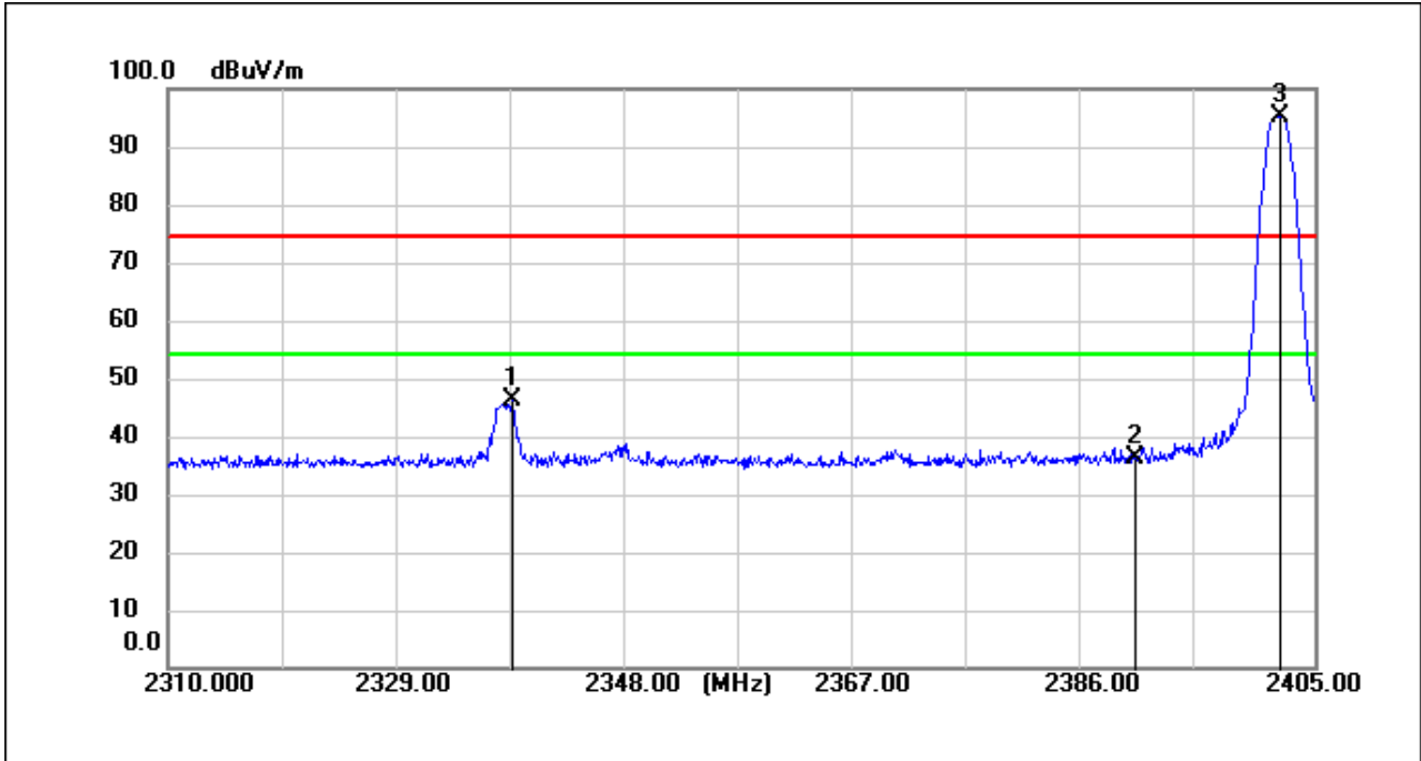
BLE_1M_TX_CH_00_Horizontal_Peak
