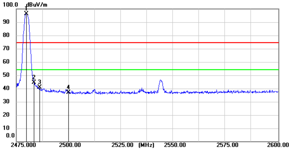
BLE_1M_TX_CH_39_Horizontal_Peak
