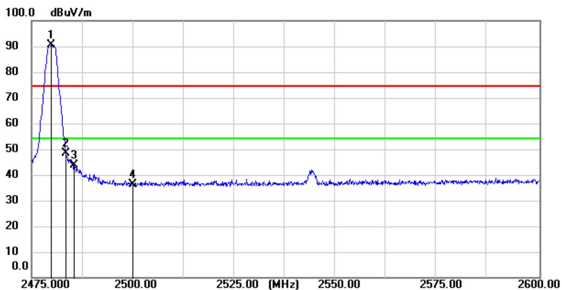
BLE_2M_TX_CH_39_Verical_Peak
