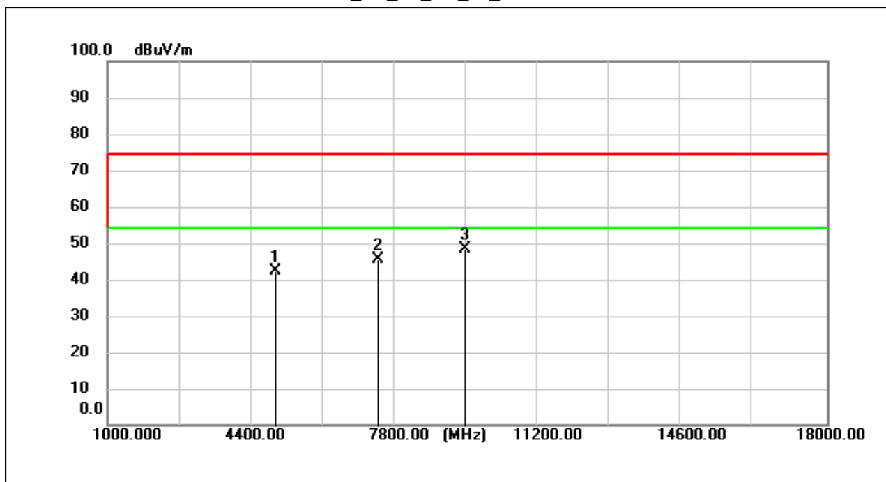
BLE_1M_TX_CH_39_Horizontal
