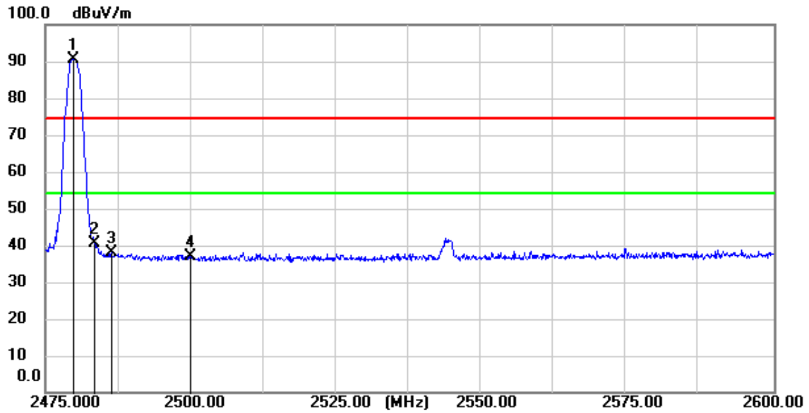
BLE_1M_TX_CH_39_Verical_Peak
