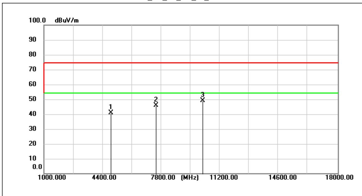
BLE_1M_TX_CH_19_Verical
