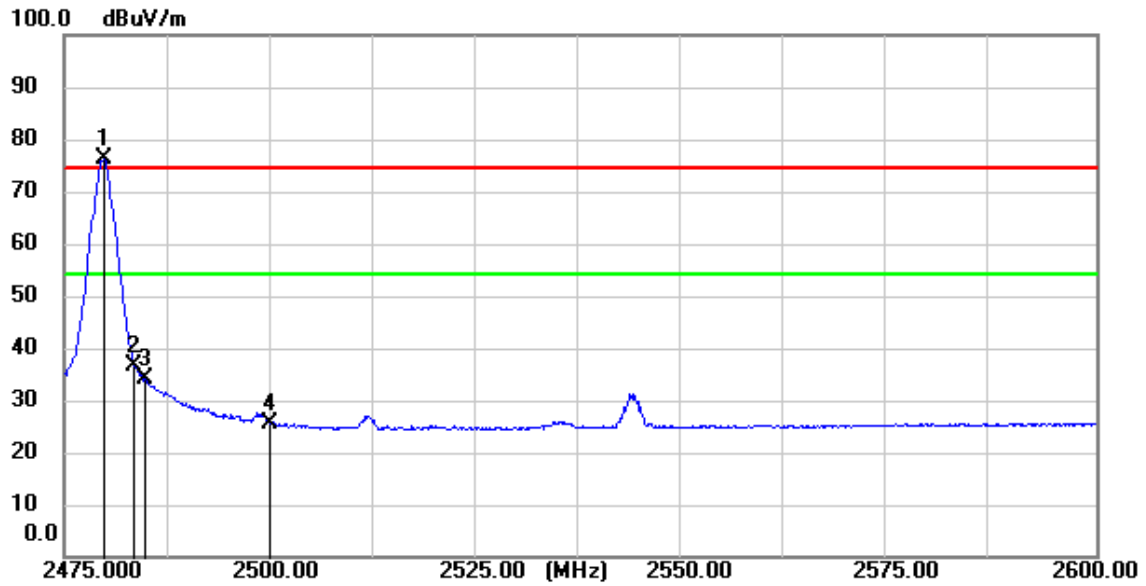
BLE_2M_TX_CH_39_Horizontal_Average
