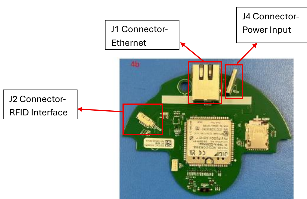
Figure 1: Top PCBA
