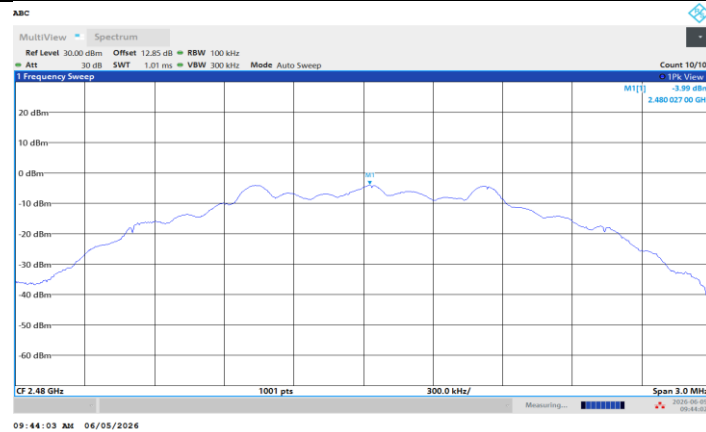
BLE_2M_Ant1_2480_0~Reference
