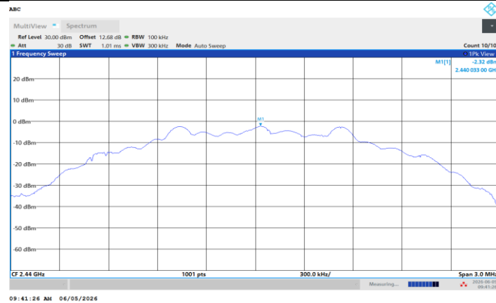
BLE_2M_Ant1_2440_0~Reference
