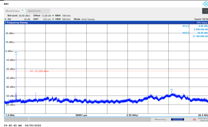
BLE_2M_Ant1_2440_1000~26500
