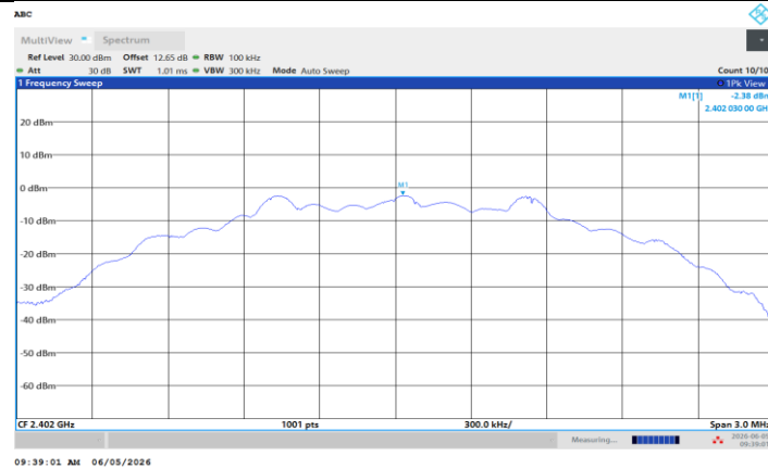
BLE_2M_Ant1_2402_0~Reference
