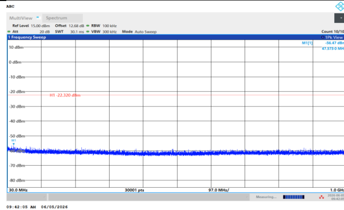
BLE_2M_Ant1_2440_30~1000
